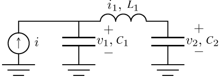
Fig. 1. Inductor-capacitor circuit in Example 1.
