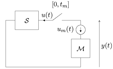
Fig. 2. Circuit diagram of an idealized measurement device \mathcal{M} and the measured system \mathcal{S} . The measurement is performed in the time interval [0, t_m] . The problem is to estimate the potential y(t_m) as well as possible, given the flow measurement u_m = -u .
