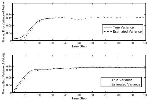
Fig. 6. Computed filtering error variance by the Riccati difference equation and the filtering error variance obtained by Monte Carlo simulations based on 500 samples.
