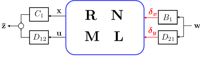
Fig. 4: The closed-loop response mapping w to \bar{z} . The SLP that maps the part of the closed-loop response that we design is the map (\delta_x, \delta_y) \rightarrow (\mathbf{x}, \mathbf{u}) .
