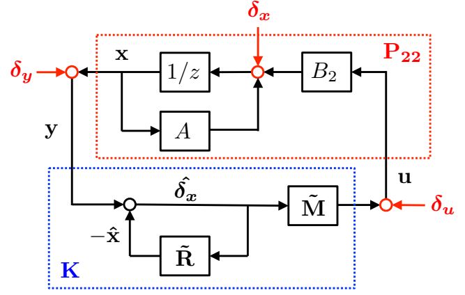
Fig. 6: Structure of the state feedback controller as described by implementation (12), where \tilde{\mathbf{R}} := I - z\mathbf{R} and \tilde{\mathbf{M}} := z\mathbf{M} .
