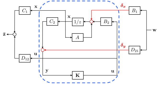
Fig. 5: Representation of the closed loop map in terms of the state space matrices from (1) and the controller \mathbf{K} . The blocks inside the dotted blue give the state space equivalent of the system response \{\mathbf{R}, \mathbf{M}, \mathbf{N}, \mathbf{L}\} .
