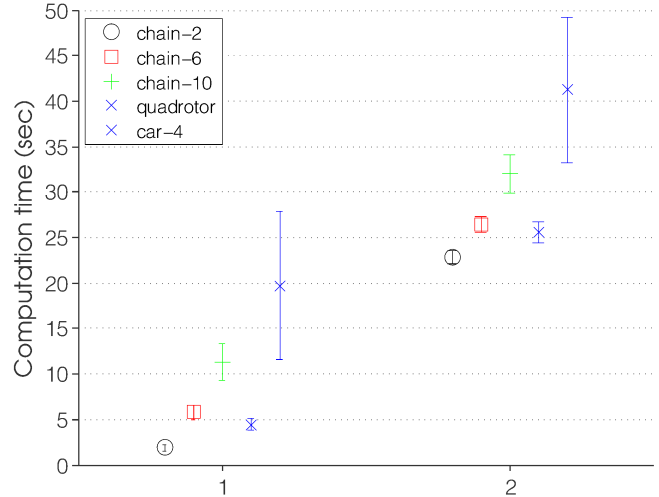
Fig. 4. Solver (1) and total (2) time (mean \pm standard error) to compute a feasible control input for various system models for the surveillance example.
