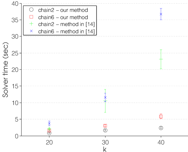
Fig. 3. Solver time (mean \pm standard error) to compute a feasible control input for the reach-avoid example with our approach and the approach in [14].
