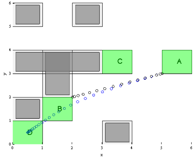
Fig. 2. Illustration of the environment for the surveillance scenario. The goals are labeled A , B , C , and D . Dark regions are obstacles. A representative trajectory for the quadrotor model is shown, where we additionally minimized an additive cost function with cost c(x_t, u_t) = |u_t| accrued at each time index.
