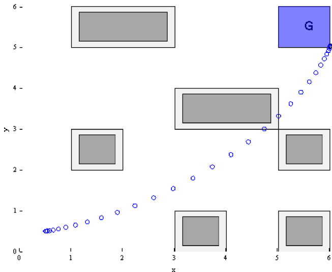
Fig. 1. Illustration of the environment for the reach-avoid scenario. The goal is labeled G and dark regions are obstacles. A representative trajectory for the “chain-6” model is shown, where we additionally minimized an additive cost function with cost c(x_t, u_t) = |u_t| accrued at each time index.
