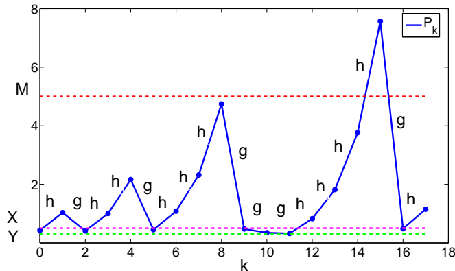
Fig. 2. A Packet Arrival Sequence
