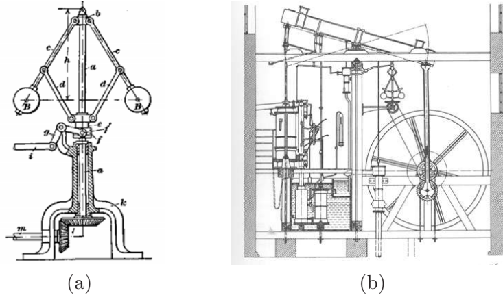
Figure 1: The centrifugal governor (a), developed in the 1780s, was an enabler of the successful Watt steam engine (b), which fueled the industrial revolution. Figures courtesy of Cambridge University.
