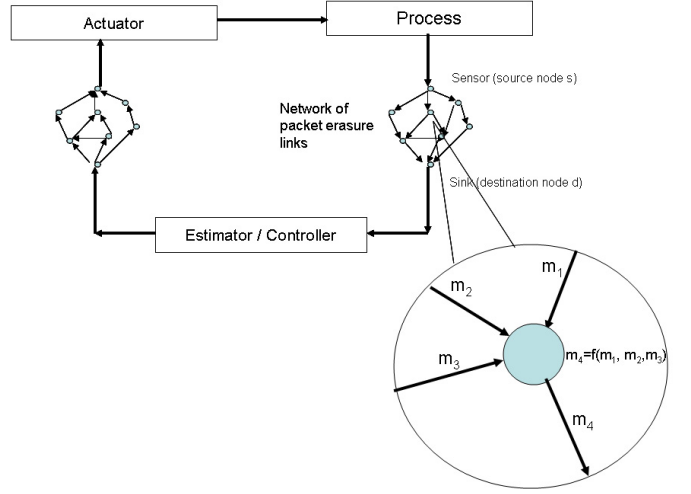
Fig. 1. The set-up of the control across communication networks problem. Every node computes a function of the incoming messages and transmits it. For most of the discussion in the paper, we ignore the network between the controller and the actuator. See, however, Remark 4.
