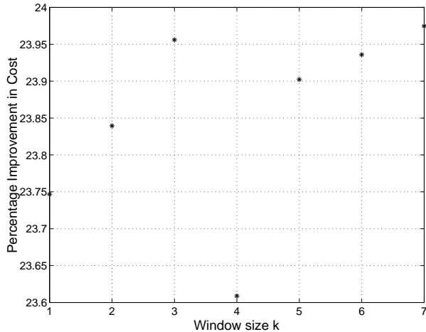
Fig. 1. Percent improvement in cost due to the optimal sensor switching strategy as predicted by the sliding window scheme.
