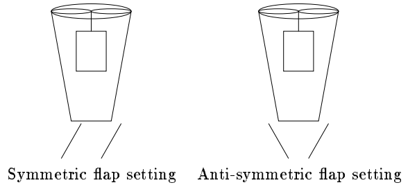
Figure 7: Two different flap settings. In both cases, the flaps are ganged. In anti-symmetric setting, the end can be closed off and apply a backward thrust at the flap angle of about 40^\circ . In symmetric setting, the fan can output a sideways force as well as a downward force.
