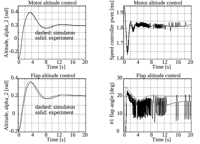
Figure 6: Comparison of altitude and control effort of the actual and the simulated data
