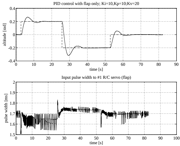
Figure 9: Set point tracking using flap control
