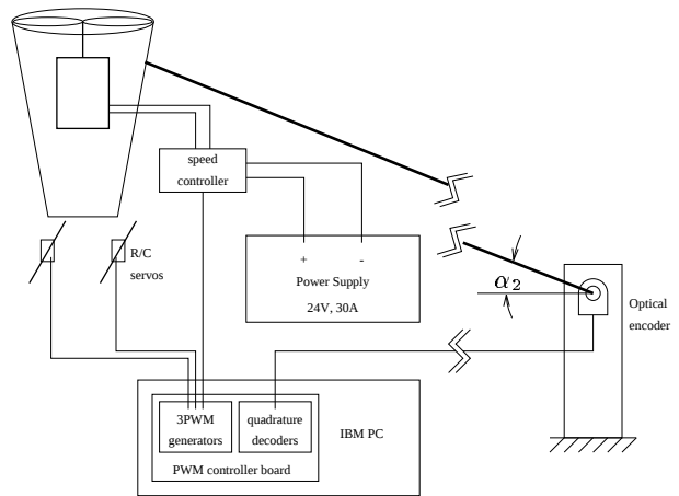
Figure 3: The computer schematic diagram
