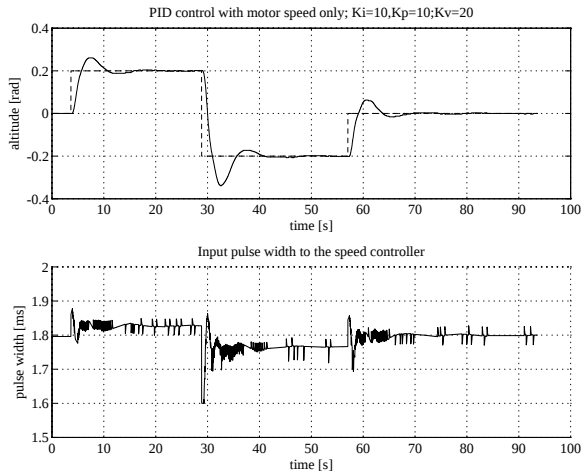
Figure 8: Set point tracking using motor control
