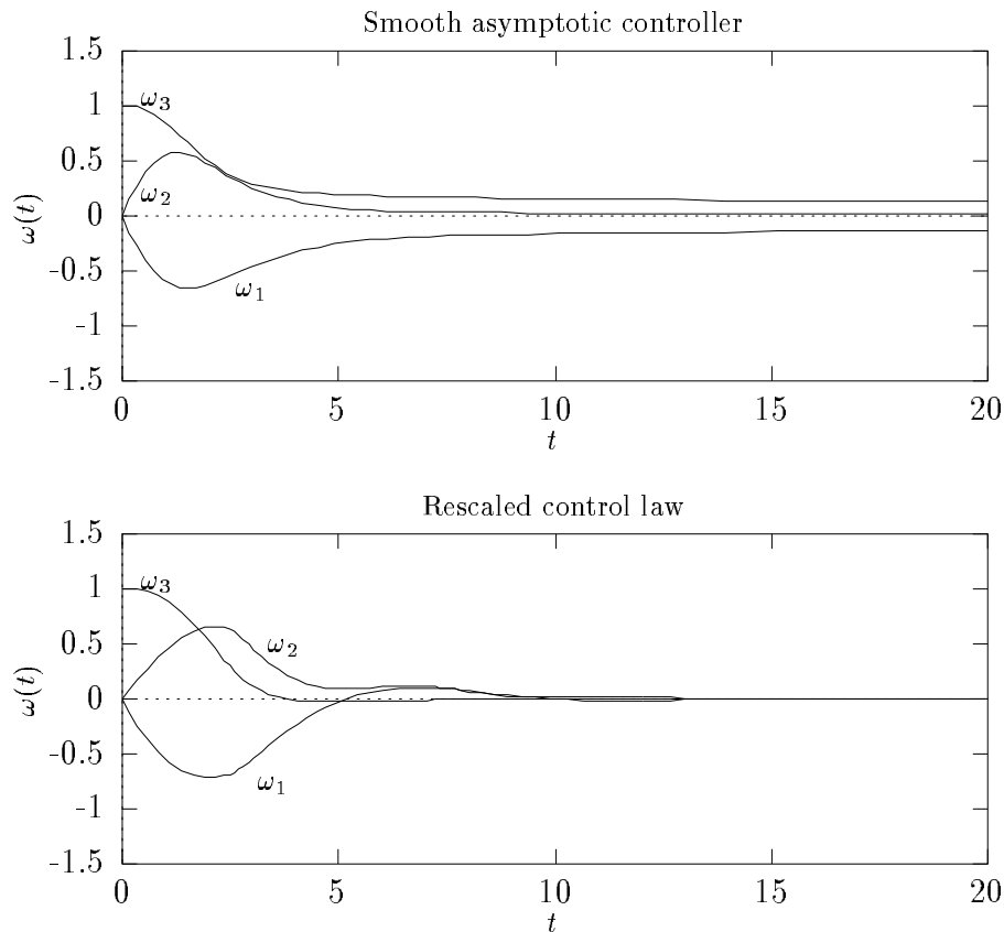
FIGURE 10. Response of the Euler equations with smooth feedback (top) and a \rho -exponential stabilizer (bottom).
