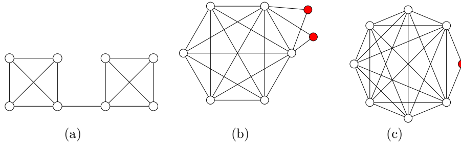
Figure 7: Graphs with the largest clustering coefficient, defining the clustering coefficient of vertices with degree d = 1 as equal to zero. (a) The optimal graph for \mathcal{G}(8, 13) has two cut vertices, connected through a bridge. (b) The smallest type II almost complete subgraph consists of a clique with N - 2 vertices, and both peripheral vertices have degree at 2. The peripheral vertices are shown in red. (c) The smallest type I almost complete graph under the new convention, where the peripheral vertex has degree 2.
