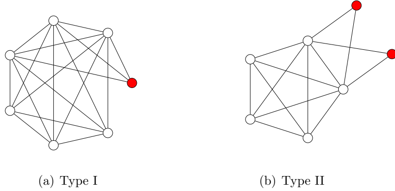
Figure 3: (a) The type I almost complete graph consists of a clique of N - 1 vertices, and one peripheral vertex (shown in red) that connects to them. (b) The type II almost complete graph of order N consists of a clique of order N - 2 , and two additional vertices that connect to it (and possibly to each other).
