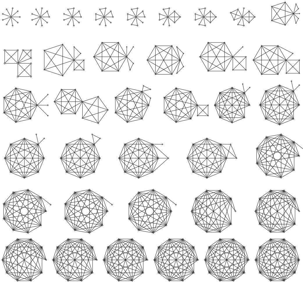
Figure 8: Graphs of order 10 and size 9 \leq m \leq 45 with the largest clustering coefficient, assuming that vertices with degree 1 have clustering coefficient equal to 1.
