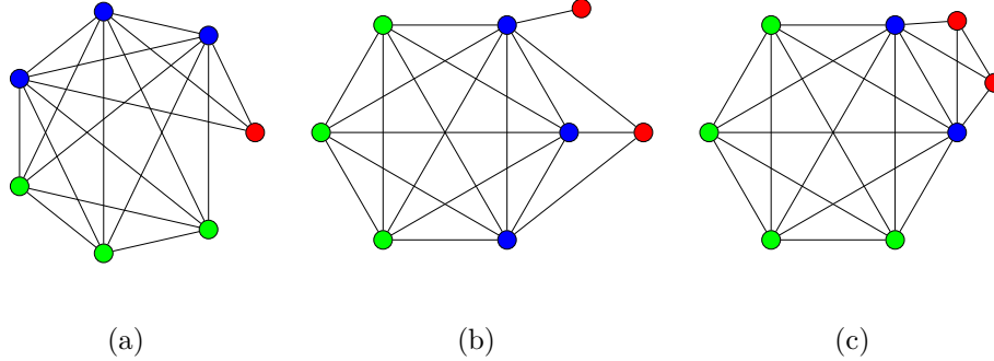
Figure 4: Clustering for the almost complete graphs. (a) The peripheral vertex (red) has unit clustering since it is connected to vertices of a clique. The vertices that are not connected to it (green) also have clustering equal to 1, as members of the complete graph with no other edges. The vertices that are connected to the peripheral vertex (blue) have clustering less than 1, since the peripheral vertex is not connected to all of their neighbors. (b) A type II almost complete graph with the largest clustering, where the two peripheral vertices are not connected (type IIa). (c) A maximum clustering coefficient type II almost complete graph, with connected peripheral vertices (type IIb).
