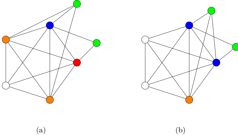
Figure 2: An example of a graph with two vertices connected to a clique. The graph in (a) has a smaller sum of clustering coefficients C_S than the one in (b). By rewiring one edge in the graph on the left, we shift the missing triangles of one orange vertex to a blue one, with a higher degree. So the missing edges between a green and a white vertex have a smaller effect on the overall clustering.
