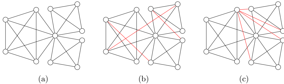
Figure 6: (a) The graph with the largest clustering coefficient of order 11 and size 22 consists of three complete subgraphs. Removal of the central vertex will render the network disconnected. (b) Addition of a few new edges among the different subgraphs creates new alternative communication paths among the various vertices of the network. As a result, the minimum cut set of the network is increased. (c) Adding new edges that connect one edge with vertices in the other subgraphs essentially creates a new network with more than one central vertex.
