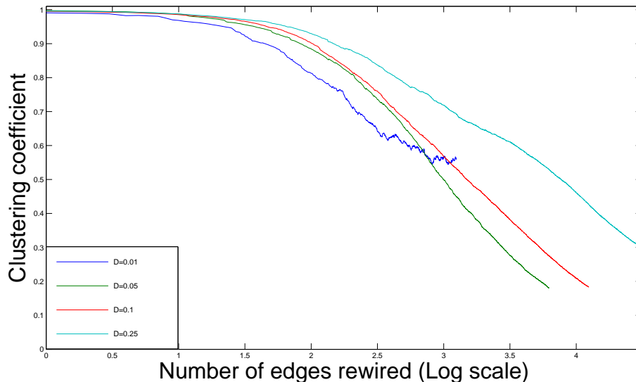
Figure 5: Typical change of the clustering coefficient of a network with N=500 vertices and various edge densities D . At every step one edge is rewired and the new average clustering coefficient is measured. We repeat the process for a number of steps equal to the number of edges in the graph. The rate of decrease in clustering is very small at first, but increases as we introduce more randomness in network architecture. Larger networks are more robust to rewiring a fixed number of edges.
