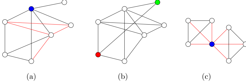
Figure 1: (a) The clustering coefficient of a vertex is the number of connections between its neighbors, divided by all pairs of neighbors, whether they are connected by an edge or not. The clustering coefficient of the blue vertex u is C(u) = 4/\binom{5}{2} = 0.4 . The average shortest path length is \bar{L}_G = 1.48 . (b) After rewiring one edge, and decreasing the distance between the red and the green vertex, the network has the smallest possible average distance, equal to 1.43. All vertex pairs now have at most a distance of 2. (c) The network with the largest possible average clustering and smallest average shortest path length. The blue vertex is the central vertex of the induced star subgraph.
