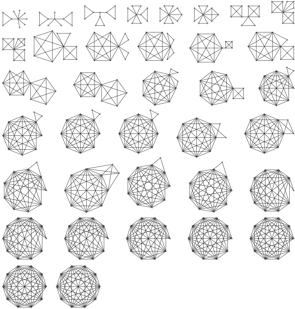
Figure 9: Graphs of order 10 and size 10 \leq m \leq 45 with the largest average clustering coefficient, assuming that vertices with degree 1 have a clustering coefficient equal to zero.
