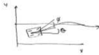
Figure 1.3: Vehicle steering using gain scheduling.
