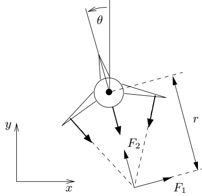
Figure 2.6: Vectored thrust aircraft (from Feedback Systems ). The net thrust on the aircraft can be decomposed into a horizontal force F_1 and a vertical force F_2 acting at a distance r from the center of mass.
