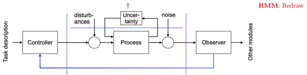
Figure 1.4: Control system standard model.
