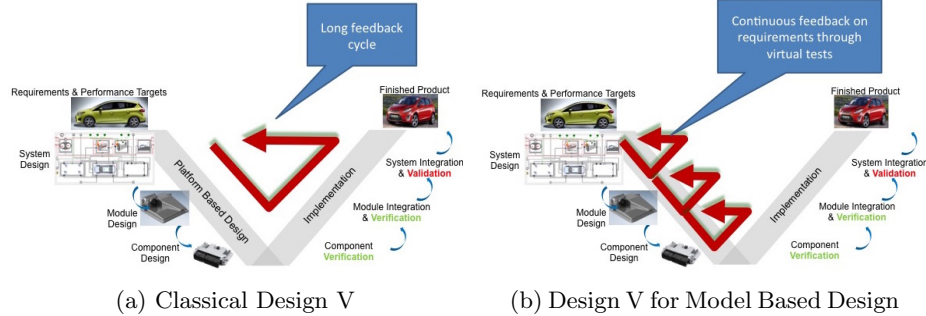
Figure 1.2: Design methodologies for complex systems. (a) The traditional design V. The left side of the V represents the decomposition of requirements and creation of system specifications. The right side represents the activities in implementation, including validation (building the right thing) and verification (building it right). Notice that validation and verification are performed late in the design process when all hardware is available. (b) A model-based design process where virtual validation is made at many stages in the design process, shortening the feedback for validation.
