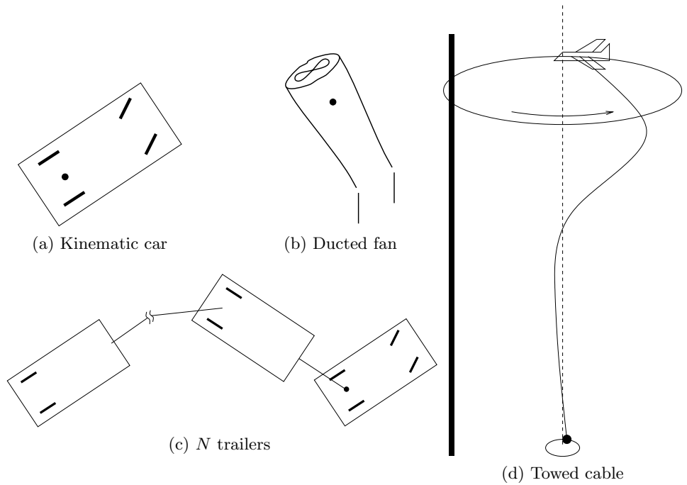
Figure 2.6: Examples of flat systems.
