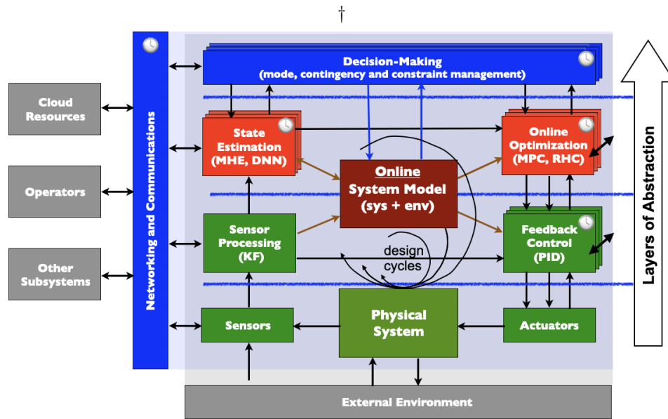
Figure 1.6: Layered control systems. The system consists of four layers: the physical layer (lowest), the feedback regulation layer (green), the trajectory generation layer (red), and the decision-making layer (blue). Networking and communications allows information to be transferred between the layers as well as with outside resources (left). The entire system interacts with the external environment, represented at the bottom of the figure.
