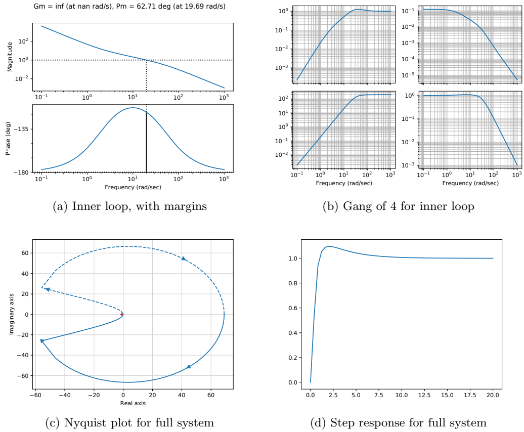
Figure 1.7: Sample outputs for PVTOL example.
