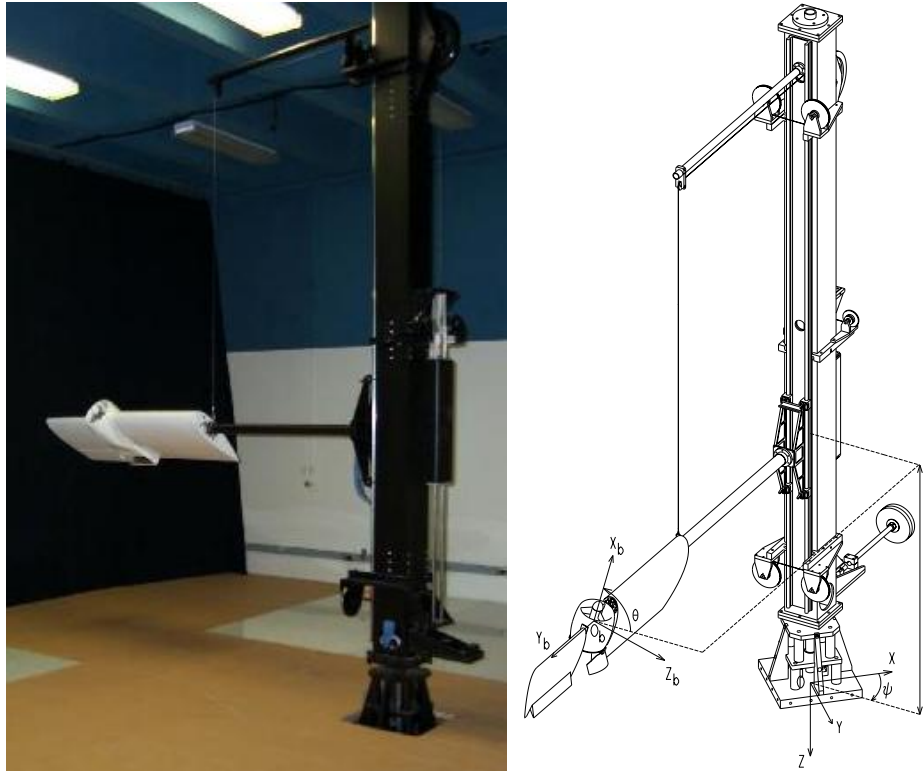
Figure 4.3: Caltech ducted fan.
