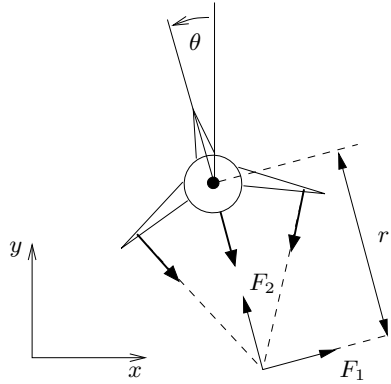
Figure 2.6: Vectored thrust aircraft (from Feedback Systems ). The net thrust on the aircraft can be decomposed into a horizontal force F_1 and a vertical force F_2 acting at a distance r from the center of mass.
