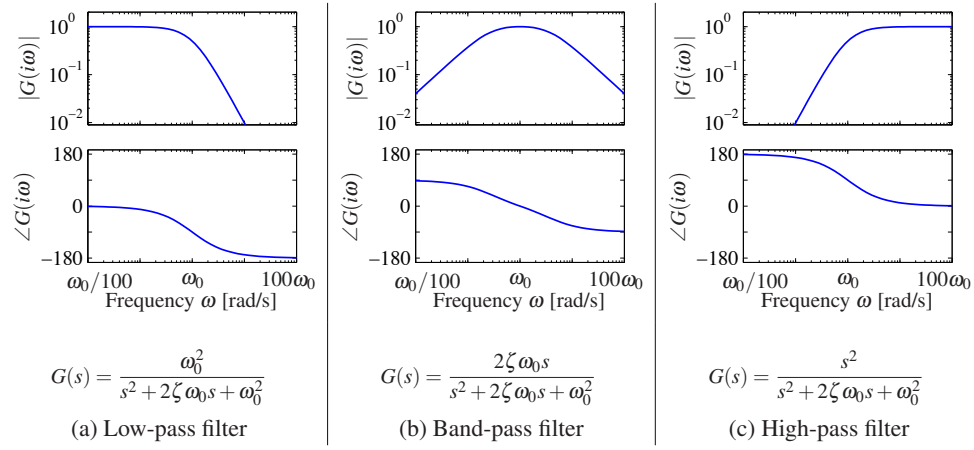
Figure 9.15: Bode plots for low-pass, band-pass and high-pass filters. The top plots are the gain curves and the bottom plots are the phase curves. Each system passes frequencies in a different range and attenuates frequencies outside of that range.
