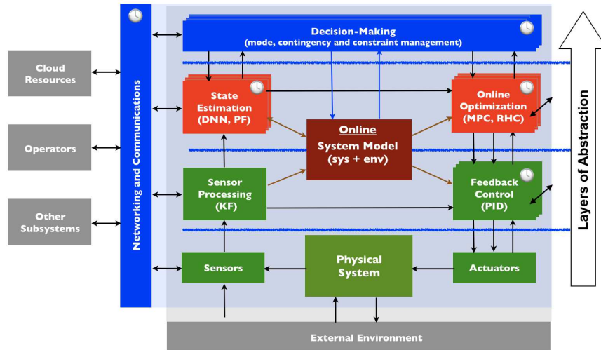
Figure 1.19: Layered decomposition of a control system.
