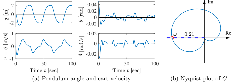
Figure 14.14: Time and frequency responses of the cart-pendulum system. (a) Time responses when the pendulum has an initial misalignment. (b) Frequency response of the transfer function G(s) (solid line), given by (14.36), and the locus of the negative inverse -1/N(a) (dashed line) of the describing function N(a) for friction, which is given by equation (14.35).
