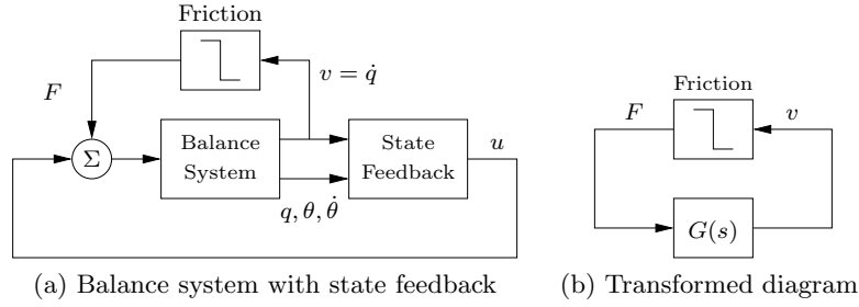
Figure 14.13: Block diagrams of a balance system with state feedback and friction. (a) Detailed block diagram showing the balance system with inputs u and F and outputs q, \theta, v = \dot{q}, \dot{\theta} . (b) Block diagram obtained after transformations. It has two blocks: the nonlinear friction block and a linear block with the transfer function G(s) from friction force F to velocity v .
