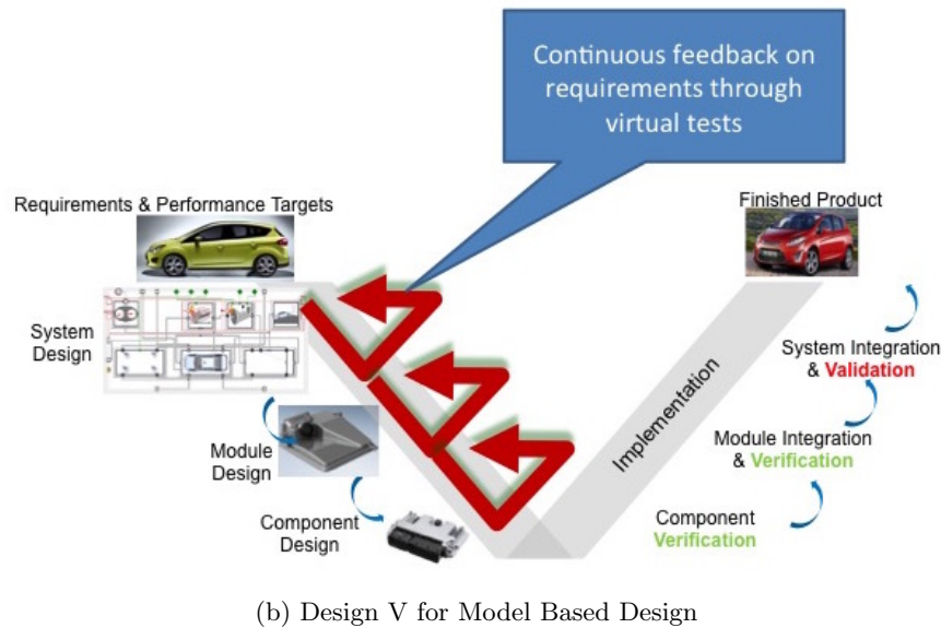
Figure 15.2: The top figure a) shows a traditional design V. The left side of the V represents the decomposition of requirements, and creation of system specifications. The right side represents the activities in implementation including validation (building the right thing) and verification (building it right). Notice that validation and verification are performed late in the design process when all hardware is available. The bottom figure b) shows a model-based design process where virtual validation is made at many stages in the design process, shortening the feedback for validation.
