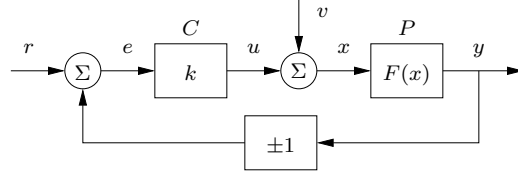
Figure 2.1: Block diagram of simple, static feedback system. The controller is a constant gain k > 0 and the process is modeled by a nonlinear function F(x) . The process output is y , the control signal is u , the external signals are the reference r , and the load disturbance v . The sign in the lower block indicates whether the feedback is positive (+) or negative (-).
