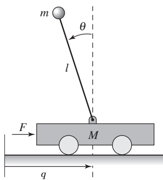
(a) Cart-pendulum system
