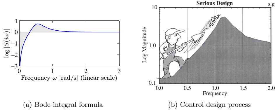
Figure 14.2: Interpretation of the waterbed effect . The function \log|S(i\omega)| is plotted versus \omega in linear scales in (a). According to Bode's integral formula (14.5), the area of \log|S(i\omega)| above zero must be equal to the area below zero. Gunter Stein's interpretation of design as a trade-off of sensitivities at different frequencies is shown in (b) (from [Ste03]).
