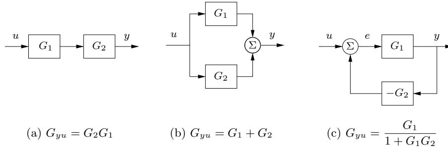
Figure 9.5: Interconnections of linear systems. Series (a), parallel (b), and feed-back (c) connections are shown. The transfer functions for the composite systems can be derived by algebraic manipulations assuming exponential functions for all signals.
