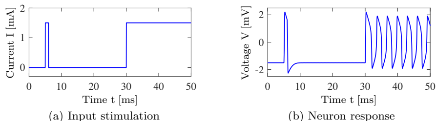
Figure 3.28: Response of a neuron to a current input. The current input is shown in (a) and the neuron voltage V in (b). The simulation was done using the FitzHugh–Nagumo model (Exercise 3.10).
