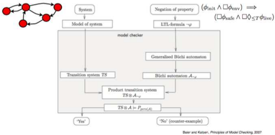
Figure 15.12: Model checking.
