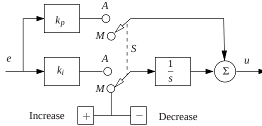
Figure 3.16: Block diagram of a PI controller that can switch between manual and automatic control. Automatic mode is indicated by A and manual mode by M. Manual control is executed by the buttons marked + and – which increase or decrease the control signal.
