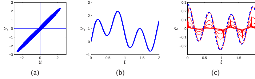
Figure 3.9: Responses of the system with integral feedback. The left plot, is a scatter plot of inputs and outputs. The center plot shows the response of the closed loop system to the input signal r , and the right plot shows the control error. The parameter variations are the same as in Figure 3.7. Notice the dramatic improvement compared to Figure 3.7b
