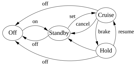
Figure 3.18: Finite state machine for cruise control system. The figure on the left shows some typical buttons used to control the system. The controller can be in one of four modes, corresponding to the nodes in the diagram on the right. Transition between the modes is controlled by pressing one of the five buttons on the cruise control interface: on, off, set, resume or cancel.
