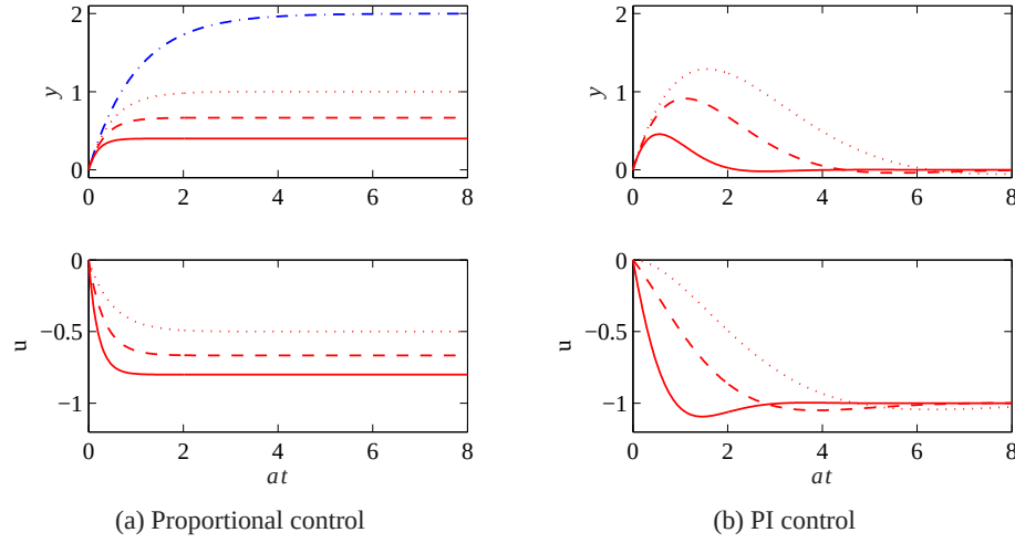
Figure 3.3: Response of open (dash-dotted) and closed loop system with prportional control (a) and PI control (b). The process transfer function is P = 2/(s+1) . The controller gains are k_p = 0.5 (dotted lines), 1 (dashed lines) and 2 (full lines) for proportional control. The PI controller is designed for (3.20) \zeta_c = 0.707 and \omega_c = 0.707 , (dotted lines) 1 (dashed lines) and 2 (full lines), which gives the controller parameters k_p = 0, 0.207, 0.914 and k_i = 0.25, 0.50 and 2.
