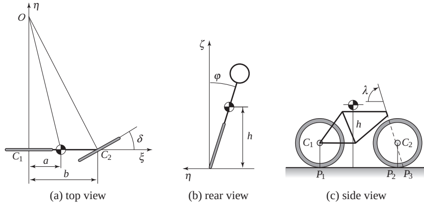
Figure A.5: Schematic views of a bicycle. The steering angle is \delta , and the roll angle is \phi . The center of mass has height h and distance a from a vertical through the contact point P_1 of the rear wheel. The wheel base b is the distance between P_1 and P_2 , and the trail c is the distance between P_2 and P_3 .
