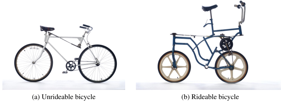
Figure 14.9: Two bicycles with rear wheel steering (a) is unrideable and (b) is rideable. Figures courtesy of Richard Klein [?].
