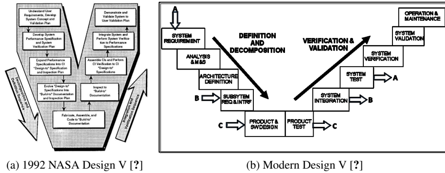
Figure 15.1: The V-model for system design. The left side of the V represents the decomposition of requirements, and creation of system specifications. The right side represents the activities in implementation including validation (building the right thing) and verification (building it right).
