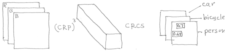
Figure 15.25: The figure is a simplified version of the convolutional neural network used for the object detection in Figure ???. The input is a color image. The output is three layers of images representing the subjective probability of finding car, bicycle, or person at a given position in the image.
