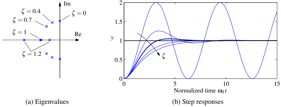
Figure 7.8: Step response for a second-order system. Normalized step responses for the system (7.23) for \zeta = 0, 0.4, 0.7 (thicker), 1 , and 1.2 . As the damping ratio is increased, the rise time of the system gets longer, but there is less overshoot. The horizontal axis is in scaled units \omega_0 t ; higher values of \omega_0 result in a faster response (rise time and settling time).
