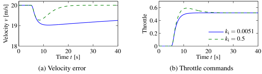
Figure 9.10: Car with PI cruise control encountering a sloping road. The velocity error is shown on the left and the throttle is shown on the right. Results with a PI controller with k_p = 0.5 and k_i = 0.0051 , where the process pole s = -0.0101 , is shown by solid lines, and a controller with k_p = 0.5 and k_i = 0.5 is shown by dashed lines. Compare with Figure 4.3b.
