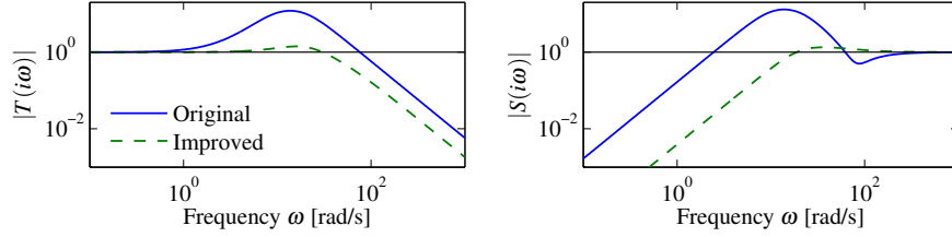
Figure 14.12: Gain curves of Bode plots for the sensitivity functions S(s) and T(s) for systems with observer-based control of vehicle steering. The plots for the original controller with \omega_c = 10 , \zeta_c = 0.707 , \omega_o = 20 , \zeta_o = 0.707 is shown in solid lines and the improved controller with \omega_c = 10 , \zeta_c = 2.6 is shown in dashed lines.
