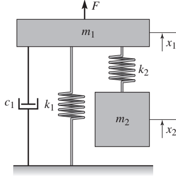
Figure 9.3: A vibration damper. Vibrations of the mass m_1 can be damped by providing it with an auxiliary mass m_2 , attached to m_1 by a spring with stiffness k_2 . The parameters m_2 and k_2 are chosen so that the frequency \sqrt{k_2/m_2} matches the frequency of the vibration.
