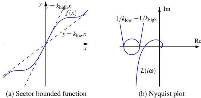
Figure 10.18: A sector bound nonlinearity (a) and illustration of the circle criterion (b).
