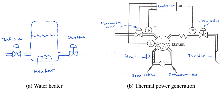
Figure 3.19: Two thermo fluid systems: (a) is a schematic diagram of a simple water heater a tank with a submerged electrical heater and (b) is a schematic of a drum boiler.
