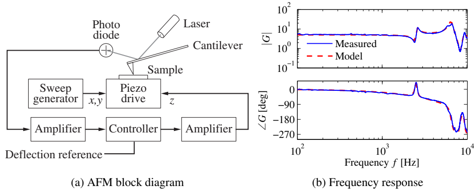
Figure 9.18: Frequency response of a preloaded piezoelectric drive for an atomic force microscope. The Bode plot shows the response of the measured transfer function (solid) and the fitted transfer function (dashed).
