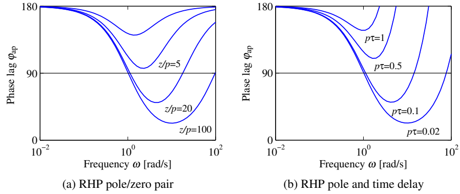
Figure 14.7: Illustration of the gain crossover frequency inequality for (a) systems with a zero and a pole in the right half-plane and (b) systems with a time delay and a right half-plane pole. The figures show the phase lag \phi_{ap} of the all-pass factor P_{ap} as a function of frequency for the systems (??). All systems have a right half-plane pole at p = 1 , both in (a) and in (b). The systems in (a) has zeros at z = 2, 5, 20 and 100 , and the systems in (b) has time delays \tau = 0.02, 0.1, 0.5 , and 1 .
