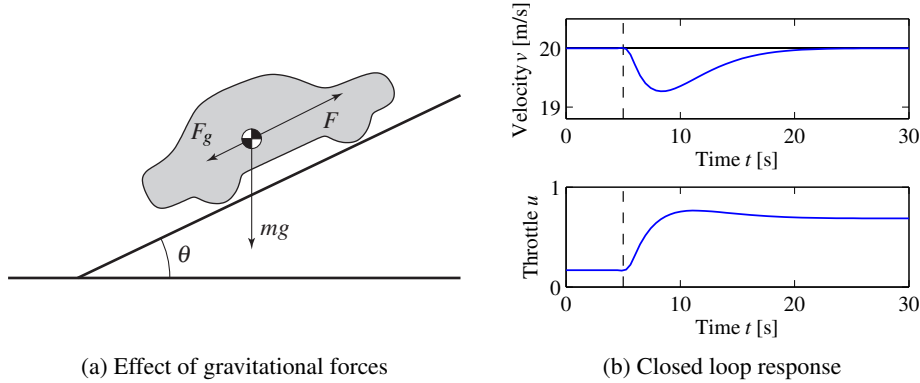
Figure 4.3: Car with cruise control encountering a sloping road. A schematic diagram is shown in (a), and (b) shows the response in speed and throttle when a slope of 4^\circ is encountered. The hill is modeled as a net change of 4^\circ in hill angle \theta , with a linear change in the angle between t = 5 and t = 6 . The PI controller has proportional gain k_p = 0.5 and integral gain k_i = 0.1 .
