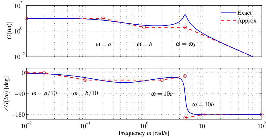
Figure 9.14: Asymptotic approximation to a Bode plot. The thin curve is the Bode plot for the transfer function G(s) = k(s+b)/(s+a)(s^2 + 2\zeta\omega_0 s + \omega_0^2) , where a \ll b \ll \omega_0 . Each segment in the gain and phase curves represents a separate portion of the approximation, where either a pole or a zero begins to have effect. Each segment of the approximation is a straight line between these points at a slope given by the rules for computing the effects of poles and zeros.
