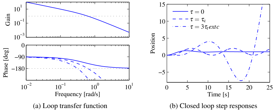
Figure 10.3: Loop transfer function and step response for the DC motor control system. The system parameters are K_m = 50 , J = 2 , c = 1 and the controller parameters are k_p = 1 and k_\tau = 0, 0.1 , and 1 .
