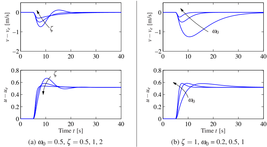
Figure 10.6: Cruise control using PI feedback. The step responses for the error and input illustrate the effect of parameters \zeta = 1 and \omega_0 on the response of a car with cruise control. The slope of the road changes linearly from 0^\circ to 4^\circ between t = 5 and 6 s. (a) Responses for \omega_0 = 0.5 and \zeta = 0.5, 1 and 2 . Choosing \zeta = 1 gives no overshoot in v . (b) Responses for \zeta = 1 and \omega_0 = 0.2, 0.5 and 1.0 .
