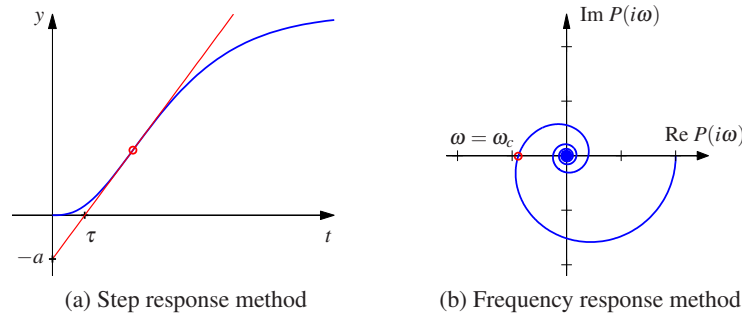
Figure 10.7: Ziegler–Nichols step and frequency response experiments. The open-loop unit step response in (a) is characterized by the parameters a and \tau . The frequency response method (b) characterizes process dynamics by the point where the Nyquist curve of the process transfer function first intersects the negative real axis and the frequency \omega_c where this occurs.
