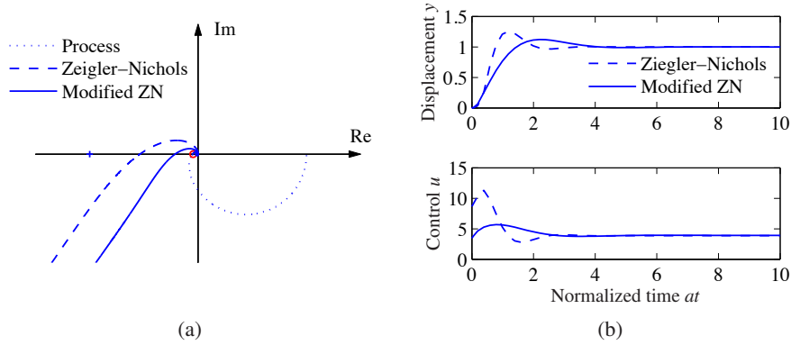
Figure 10.8: PI control of an AFM in tapping mode. Nyquist plots (a) and step responses (b) for PI control of the vertical motion of an atomic force microscope in tapping mode. Results with Ziegler–Nichols tuning are shown by dashed lines, and modified Ziegler–Nichols tuning is shown by solid lines. The Nyquist plot of the process transfer function is shown by dotted lines.
