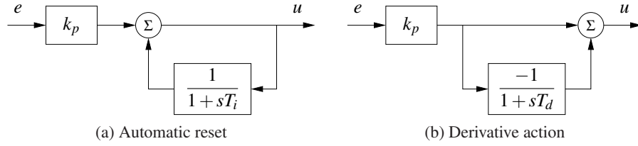
Figure 10.3: The block diagram in (a) shows how integral action is implemented using positive feedback with a first-order system, sometimes called automatic reset . The block diagram in (b) shows how derivative action can be implemented by taking differences between a static system and a first-order system.
