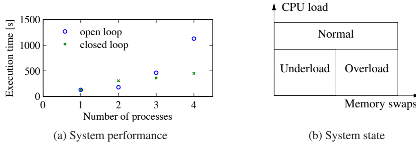
Figure 2.22: Illustration of feedback in the virtual memory system of the IBM/370. (a) The effect of feedback on execution times in a simulation, following [BG68]. Results with no feedback are shown with \circ , and results with feedback with \times . Notice the dramatic decrease in execution time for the system with feedback. (b) How the three states are obtained based on process measurements.
