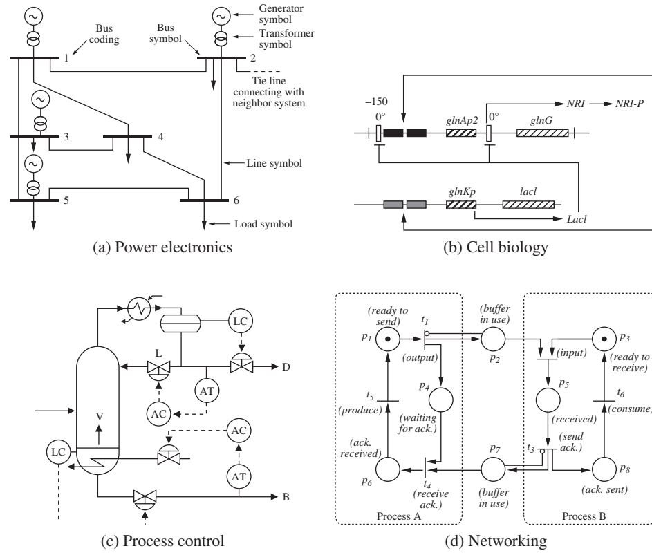
Figure 2.13: Schematic diagrams for different disciplines. Each diagram is used to illustrate the dynamics of a feedback system: (a) electrical schematics for a power system [Kun93], (b) a biological circuit diagram for a synthetic clock circuit [ASMN03], (c) a process diagram for a distillation column [SEM04] and (d) a Petri net description of a communication protocol.
