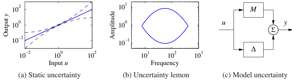
Figure 2.17: Characterization of model uncertainty. Uncertainty of a static system is illustrated in (a), where the solid line indicates the nominal input/output relationship and the dashed lines indicate the range of possible uncertainty. The uncertainty lemon [GPD59] in (b) is one way to capture uncertainty in dynamical systems emphasizing that a model is valid only in the amplitude and frequency ranges within the shaded region. In (c) a model is represented by a nominal model M and another model \Delta representing the uncertainty analogous to the representation of parameter uncertainty.
