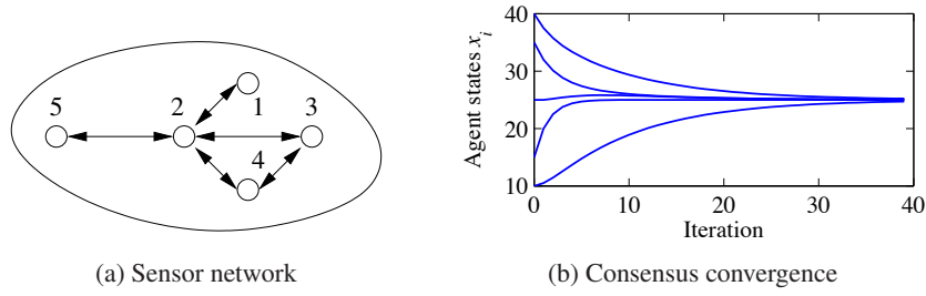
Figure 2.23: Consensus protocols for sensor networks. (a) A simple sensor network with five nodes. In this network, node 1 communicates with node 2 and node 2 communicates with nodes 1, 3, 4, 5, etc. (b) A simulation demonstrating the convergence of the consensus protocol (2.32) to the average value of the initial conditions.
