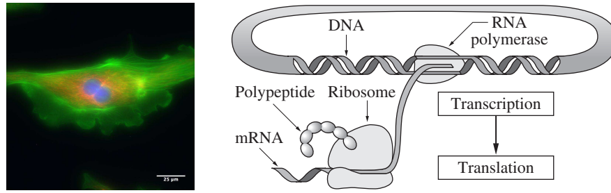
Figure 2.24: Biological circuitry. The cell on the left is a bovine pulmonary cell, stained so that the nucleus, actin and chromatin are visible. The figure on the right gives an overview of the process by which proteins in the cell are made. RNA is transcribed from DNA by an RNA polymerase enzyme. The RNA is then translated into a polypeptide chain by a molecular machine called a ribosome, and then the polypeptide chain folds into a protein molecule.
