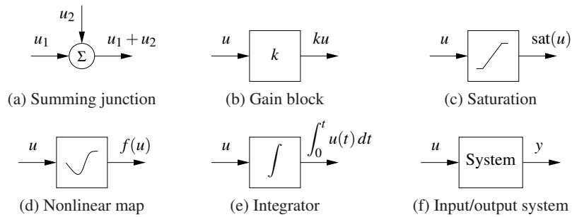
Figure 2.14: Standard block diagram elements. The arrows indicate the inputs and outputs of each element, with the mathematical operation corresponding to the block labeled at the output. The system block (f) represents the full input/output response of a dynamical system.
