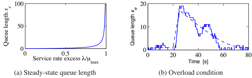
Figure 2.21: Queuing dynamics. (a) The steady-state queue length as a function of \lambda/\mu_{\max} . (b) The behavior of the queue length when there is a temporary overload in the system. The solid line shows a realization of an event-based simulation, and the dashed line shows the behavior of the flow model (2.30). The maximum service rate is \mu_{\max} = 1 , and the arrival rate starts at \lambda = 0.5 . The arrival rate is increased to \lambda = 4 at time 20, and it returns to \lambda = 0.5 at time 25.
