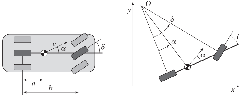
Figure 2.18: Vehicle steering dynamics. The left figure shows an overhead view of a vehicle with four wheels. The wheel base is b and the center of mass at a distance a forward of the rear wheels. By approximating the motion of the front and rear pairs of wheels by a single front wheel and a single rear wheel, we obtain an abstraction called the bicycle model , shown on the right. The steering angle is \delta and the velocity at the center of mass has the angle \alpha relative the length axis of the vehicle. The position of the vehicle is given by (x, y) and the orientation (heading) by \theta .
