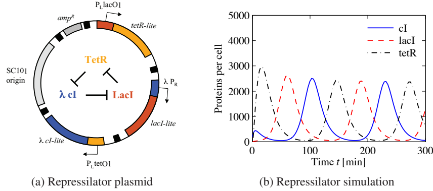
Figure 2.25: The repressilator genetic regulatory network. (a) A schematic diagram of the repressilator, showing the layout of the genes in the plasmid that holds the circuit as well as the circuit diagram (center). (b) A simulation of a simple model for the repressilator, showing the oscillation of the individual protein concentrations. (Figure courtesy M. Elowitz.)
