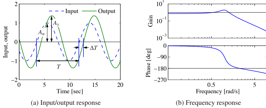
Figure 5.11: Steady-state response of an asymptotically stable linear system to a sinusoid. (a) A sinusoidal input of magnitude A_u (dashed) gives a sinusoidal output of magnitude A_y (solid), delayed by \Delta T seconds. (b) Frequency response, showing gain and phase. The gain is given by the ratio of the output amplitude to the input amplitude, M = A_y/A_u . The phase lag is given by \theta = -2\pi\Delta T/T ; it is negative for the case shown because the output lags the input.
