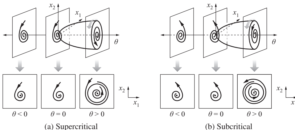
Figure 3.21: Hopf bifurcation. (a) As \theta increases a stable limit cycle appears. (b) As \theta increases a periodic orbit appears but it is unstable. Figure reproduced from [100]; used with permission.
