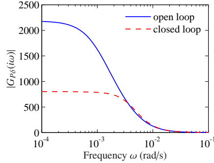
Figure 3.7: Attenuation of perturbations in a genetic circuit with linearization given by equation (3.8). The parameters of the closed loop system are given by \alpha = 800 \mu\text{M/s} , \alpha_0 = 5 \times 10^{-4} \mu\text{M/s} , \gamma = 0.001 \text{ s}^{-1} , \delta_0 = 0.005 \text{ s}^{-1} , \kappa = 0.02 \text{ s}^{-1} , n = 2 , and K = 0.025 \mu\text{M} . For the open loop system, we have set \alpha = P_e \delta_0 / (\kappa / \gamma) to make the steady state values of open loop and closed loop systems the same.
