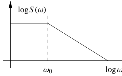
Figure 4.4: Spectral power density for a first-order Markov process.
