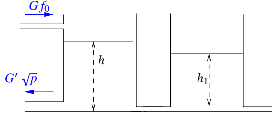
Figure 7.9: We amplify the input flow f_0 through a large gain G and we apply a large negative feedback by employing a large output pipe with output flow G' \sqrt{p} .
