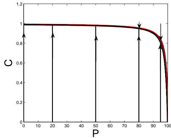
Figure 3.13: The slow manifold of the system C = g(P) is shown in red. In black, we show the trajectories of the full system. These trajectories collapse into an \epsilon -neighbor of the slow manifold. Here, we have S_{tot} = 100 , E_{tot} = 1 , k_r = k_f = 10 , and k_{cat} = 0.1 .
