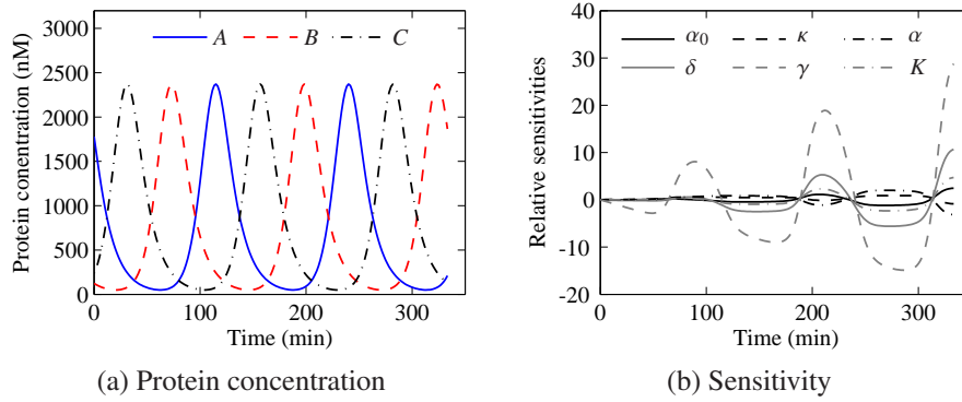
Figure 5.7: Repressor parameter sensitivity analysis. (a) Protein concentrations as functions of time. (b) Sensitivity plots. The most important parameters are the protein and mRNA decay rates \gamma and \delta . Parameter values used in the simulations are \alpha = 800 nM/s, \alpha_0 = 5 \times 10^{-4} nM/s, \delta = 5.78 \times 10^{-3} s ^{-1} , \gamma = 1.16 \times 10^{-3} s ^{-1} , \kappa = 0.116 s ^{-1} , n = 2 , and K = 1600 nM.
