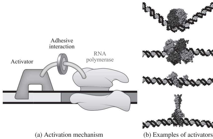
Figure 2.12: Activation of gene expression. (a) Conceptual operation of an activator. The activator binds to DNA upstream of the gene and attracts RNA polymerase to the DNA strand. (b) Examples of activators: catabolite activator protein (CAP), p53 tumor suppressor, zinc finger DNA binding domain and leucine zipper DNA binding domain. Figures adapted from Phillips, Kondev and Theriot [78]. Copyright 2009 from Physical Biology of the Cell by Phillips et al. Reproduced by permission of Garland Science/Taylor & Francis LLC.
