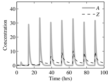
Figure 6.20: Simulation results for the concentration of protein Z in Figure 6.19 in the case in which this were used directly as an input to the downstream system, thus binding sites p' (dashed plot). The clock parameters are the same as those in Figure 6.2c and \gamma_K = \gamma_A .
