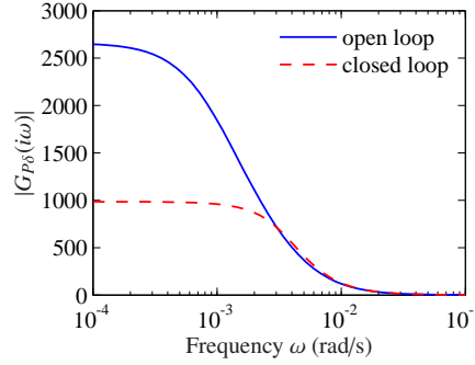
Figure 3.7: Attenuation of perturbations in a genetic circuit with linearization given by equation (3.8). The parameters of the closed loop system are given by \alpha = 800 \text{ } \mu\text{M/s} , \alpha_0 = 5 \times 10^{-4} \text{ } \mu\text{M/s} , \gamma = 0.001 \text{ s}^{-1} , \delta_0 = 0.005 \text{ s}^{-1} , \kappa = 0.02 \text{ s}^{-1} , n = 2 , and K = 0.025 \text{ } \mu\text{M} . For the open loop system, we have set \alpha = P_e \delta_0 / (\kappa / \gamma) to make the steady state values of open loop and closed loop systems the same.
