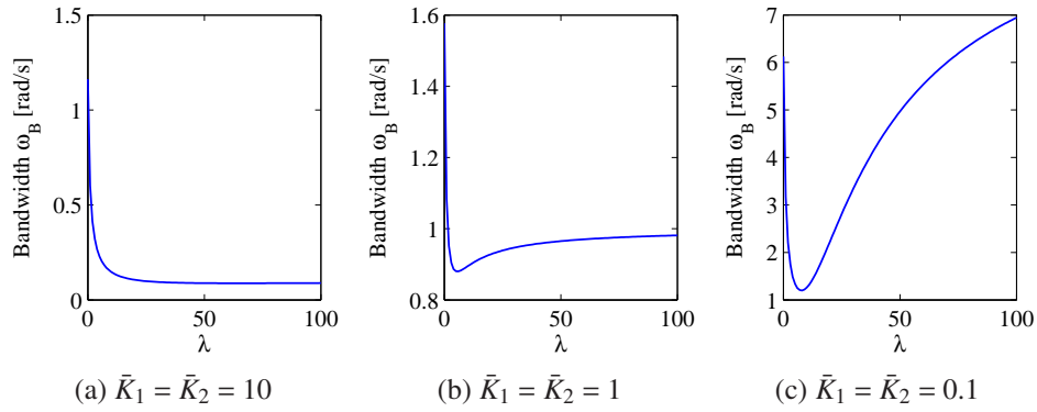
Figure 6.9: Behavior of the bandwidth as a function of the effective load \lambda for different values of the constants \bar{K}_1, \bar{K}_2 .
