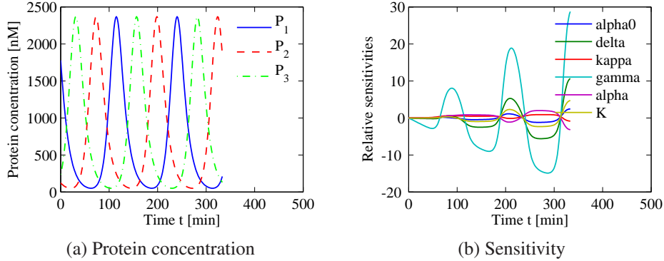
Figure 5.7: Repressilator parameter sensitivity analysis. (a) Protein concentrations as functions of time. (b) Sensitivity plots. The most important parameters are the protein and mRNA decay rates \gamma and \delta . Parameter values used in the simulations are \alpha = 800 nM/s, \alpha_0 = 5 \times 10^{-4} nM/s, \delta = 5.78 \times 10^{-3} s -1 , \gamma = 1.16 \times 10^{-3} s -1 , \kappa = 0.116 s -1 , n = 2 , and K = 1600 nM.
