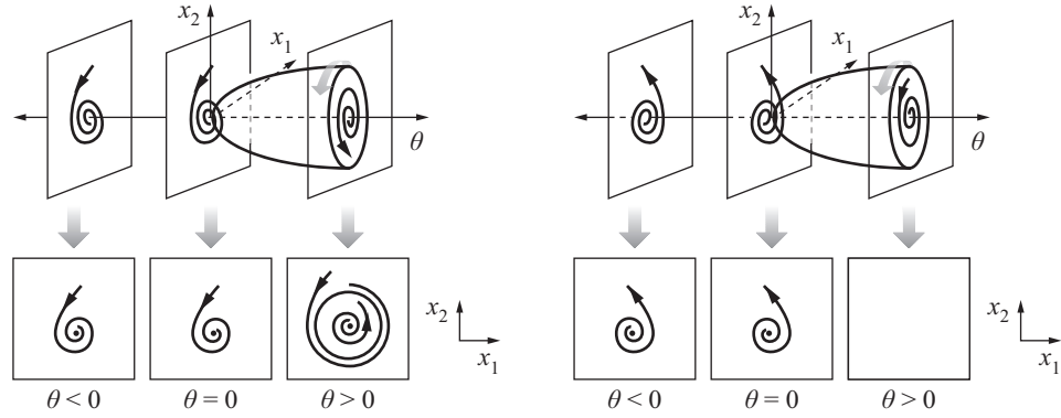
Figure 3.21: Hopf bifurcation. On the left-hand side, as \theta increases a stable limit cycle appears. On the right-hand side, as \theta increases a limit cycle appears but it is unstable. Figure taken from [98].
