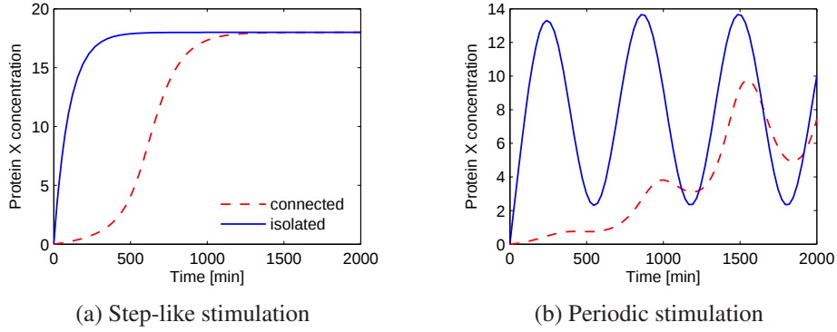
Figure 6.5: The effect of retroactivity. The solid line represents X(t) originating by equations (6.2), while the dashed line represents X(t) obtained by equation (6.3). Both transient and permanent behaviors are different. Here, k(t) = 0.18 in (a) and k(t) = 0.01(8 + 8\sin(\omega t)) with \omega = 0.01 \text{ min}^{-1} in (b). The parameter values are given by k_{\text{on}} = 10 \text{ min}^{-1}\text{nM}^{-1} , k_{\text{off}} = 10 \text{ min}^{-1} , \gamma = 0.01 \text{ min}^{-1} , and p_{\text{tot}} = 100 \text{ nM} . The frequency of oscillations is chosen to have a period of about 11 hours in accordance to what is experimentally observed in the synthetic clock of [6].
