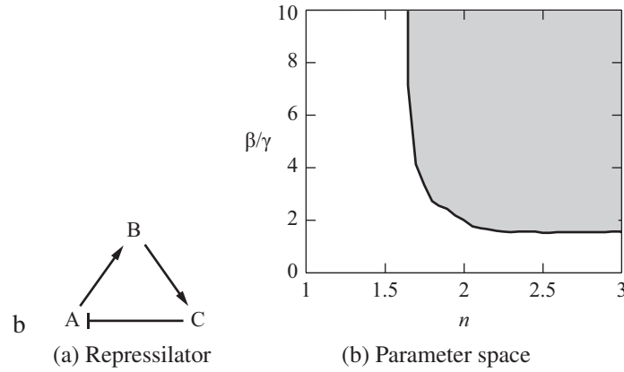
Figure 5.5: Parameter space for the repressilator. (a) Repressilator diagram. (b) Space of parameters that give rise to oscillations. Here, we have set K = 1 for simplicity.
