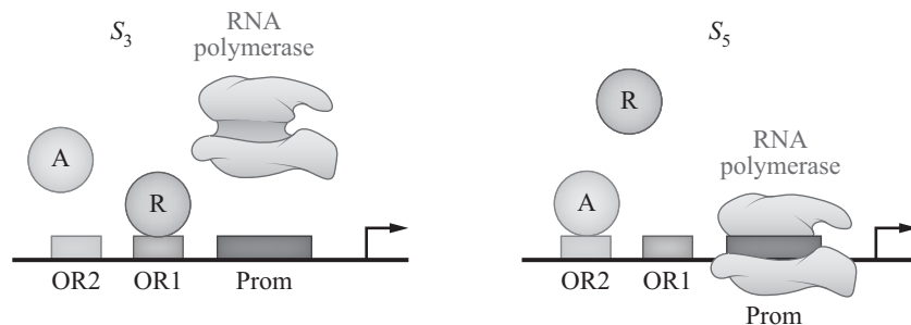
Figure 4.2: Two possible configurations of a combinatorial promoter where both an activator and a repressor can bind to specific operator sites. We show configurations S_3 and S_5 referring to Table 4.1.
