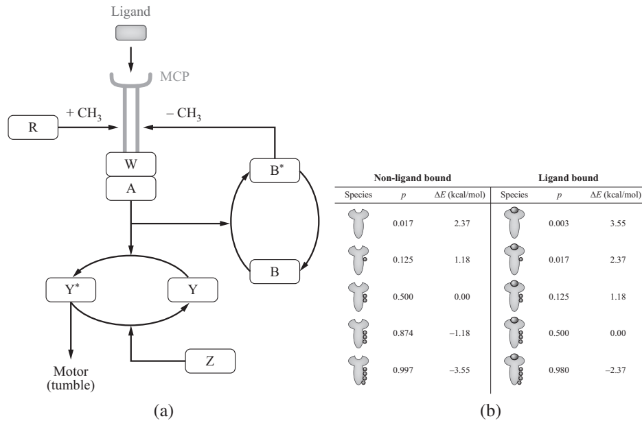
Figure 5.15: Control system for chemotaxis. (a) The sensing system is implemented by the receptor complex, which detects the presence of a ligand in the cell's outer environment. The computation part is implemented by a combined phosphorylation/methylation process, which realizes a form of integral feedback. The actuation component is realized by the CheY phosphorylated protein controlling directly the direction in which the motor spins. Figure from Rao et al. [81] (Figure 1A). (b) Receptor complex states. The probability of a given state being in an active configuration is given by p . \Delta E represents the difference in energy levels from a reference state. Figure obtained from [70].
