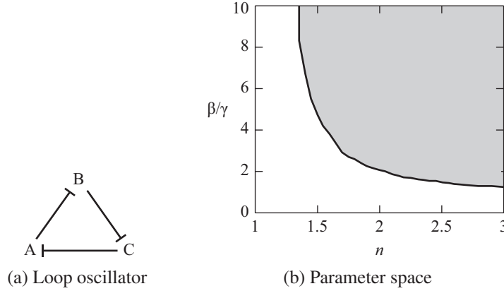
Figure 5.6: Parameter space for a loop oscillator. (a) Oscillator diagram. (b) Space of parameters that give rise to oscillations. As the value of n is increased, the range of the other parameter for which a periodic cycle exists becomes larger. Here, we have set K = 1 .
