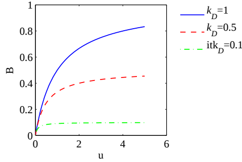
Figure 5.12: Behavior of the equilibrium value of B as a function of the input u . Concentration is in \mu\text{M} .
