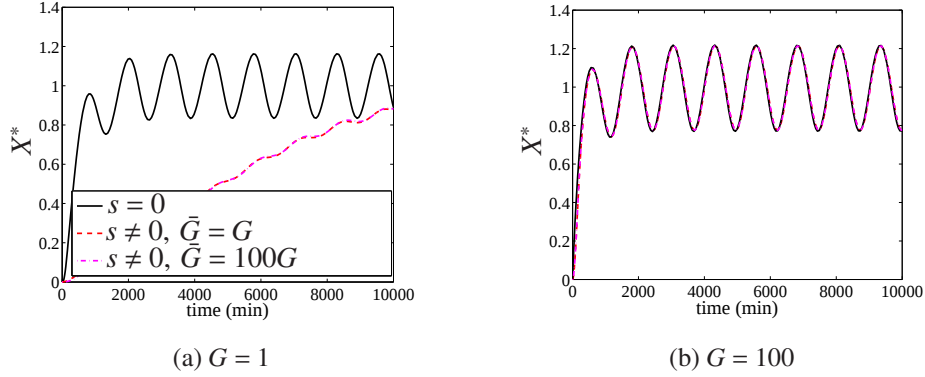
Figure 6.18: Output response of the phosphotransfer system with a periodic signal k(t) = \gamma(1 + 0.5 \sin \omega t) . The parameters are given by \gamma = 0.01 \text{ min}^{-1} , X_{\text{tot}} = 5000 \text{ nM} , k_1 = k_2 = k_3 = k_4 = 0.01 \text{ min}^{-1} \text{ nM}^{-1} , \pi_1 = \pi_2 = 0.01G \text{ min}^{-1} in which G = 1 in (a), and G = 100 in (b). The downstream system parameters are given by K_d = 1 \text{ nM} and k_{\text{off}} = 0.01\bar{G} \text{ min}^{-1} , in which \bar{G} takes the values indicated in the legend. The isolated system ( s = 0 ) corresponds to p_{\text{tot}} = 0 while the connected system ( s \neq 0 ) corresponds to p_{\text{tot}} = 100 \text{ nM} .
