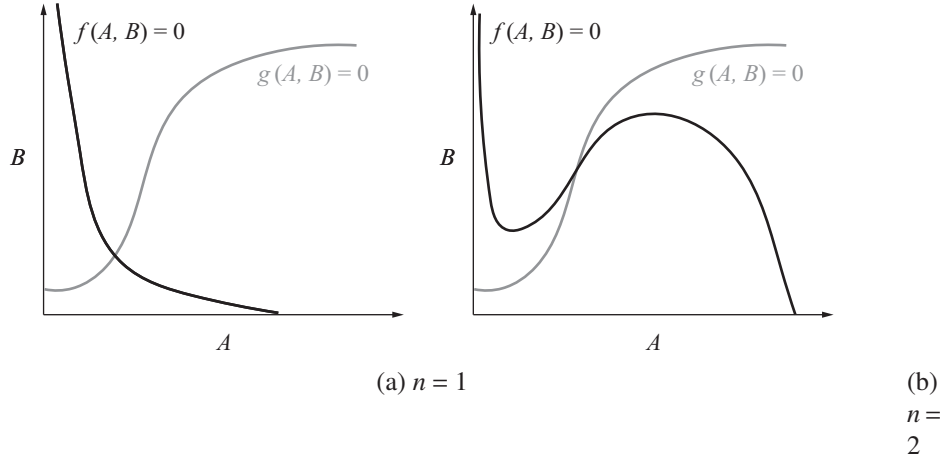
Figure 5.8: Nullclines for the two-dimensional system (5.11). (a) shows the only possible configuration of the nullclines when n = 1 . (b) shows a possible configuration of the nullclines when n = 2 . In this configuration, there is a unique equilibrium, which can be unstable.
