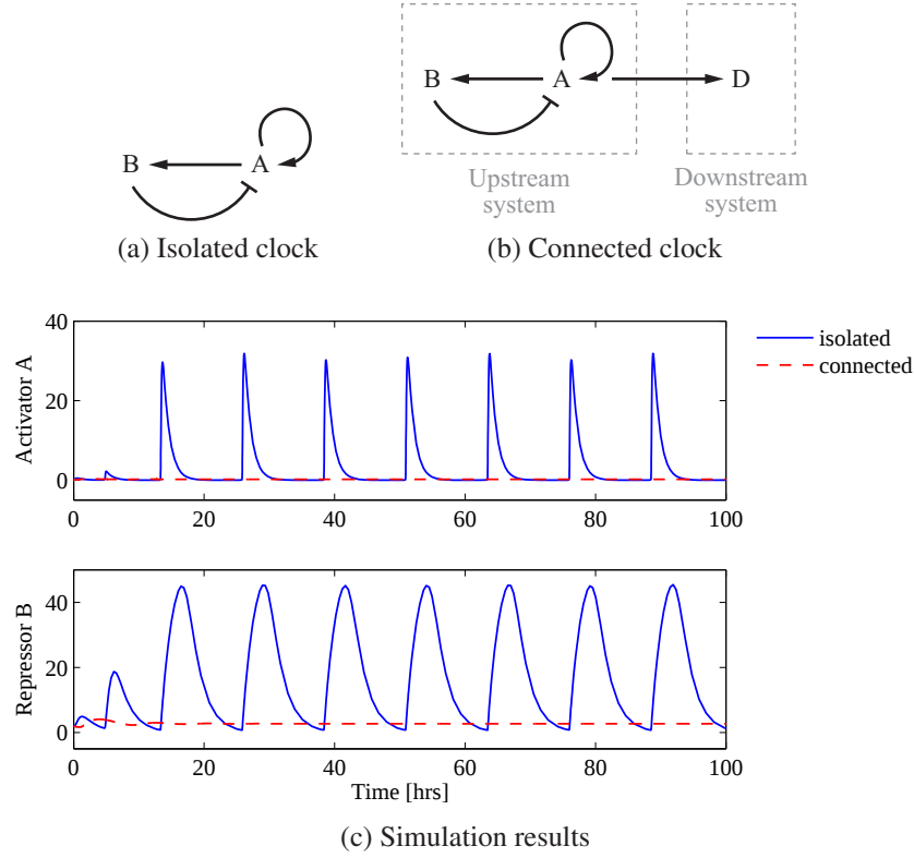
Figure 6.2: Interconnection of an activator-repressor clock to a downstream system. (a) The activator-repressor clock is isolated. (b) The clock is connected to a downstream system. (c) When the clock is connected, periodic behavior of the proteins concentrations is lost and oscillations are quenched. The clock hence fails to transmit the desired periodic stimulation to the downstream system. In all simulations, we have chosen the parameters of the clock as in Figure 5.9. For system in (b), we added the reversible binding reaction of A with sites p in the downstream system: nA + p \rightleftharpoons C with conservation law p_{\text{tot}} = p + C , with p_{\text{tot}} = 5\text{nM} , association rate constant k_{\text{on}} = 50 \text{ min}^{-1} \text{ nM}^{-n} , and dissociation rate constant k_{\text{off}} = 50 \text{ min}^{-1} (see Exercise 6.12).
