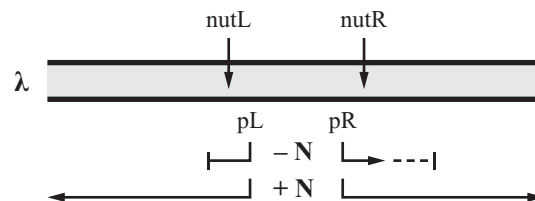
Figure 2.16: Antitermination. Protein N binds to DNA regions labeled nut , enabling transcription of longer DNA sequences. Reproduced from [37].
