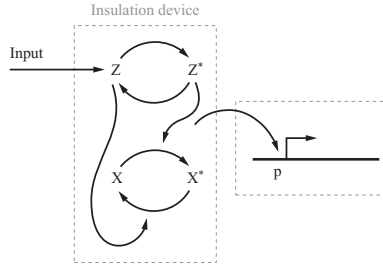
Figure 6.17: The insulation device is a phosphotransfer system. The output X^* activates transcription through the reversible binding of X^* to downstream DNA promoter sites p .
