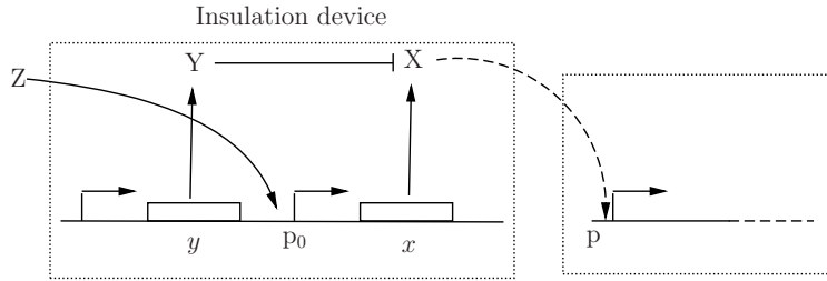
Figure 6.12: Implementation of high gain feedback (Design 1). The input Z(t) is amplified by virtue of a strong promoter p_0 . The negative feedback on the output X is obtained by enhancing its degradation through the protease Y .
