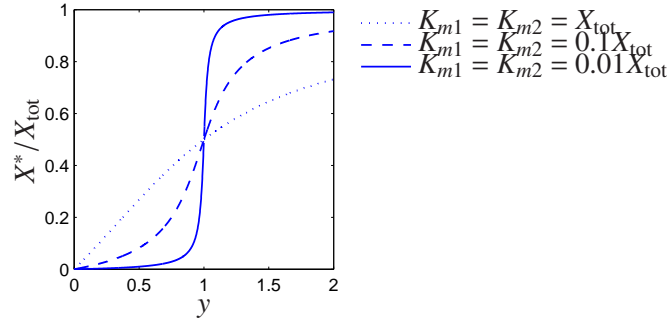
Figure 2.24: Steady state characteristic curve of a covalent modification cycle as a function of the Michaelis-Menten constants K_{m,1} and K_{m,2} .
