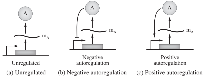
Figure 2.17: Autoregulation of gene expression. In (a) the circuit is unregulated, while (b) shows negative autoregulation and (c) shows positive autoregulation.
