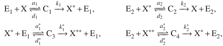
Figure 2.28: Schematic representation of a double phosphorylation cycle. E_1 is the input and X^{**} is the output.
