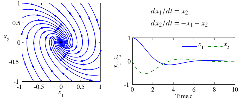
Figure 3.2: Phase portrait and time domain simulation for a system with a single asymptotically stable equilibrium point. The equilibrium point x_e at the origin is asymptotically stable since the trajectories converge to this point as t \rightarrow \infty .
