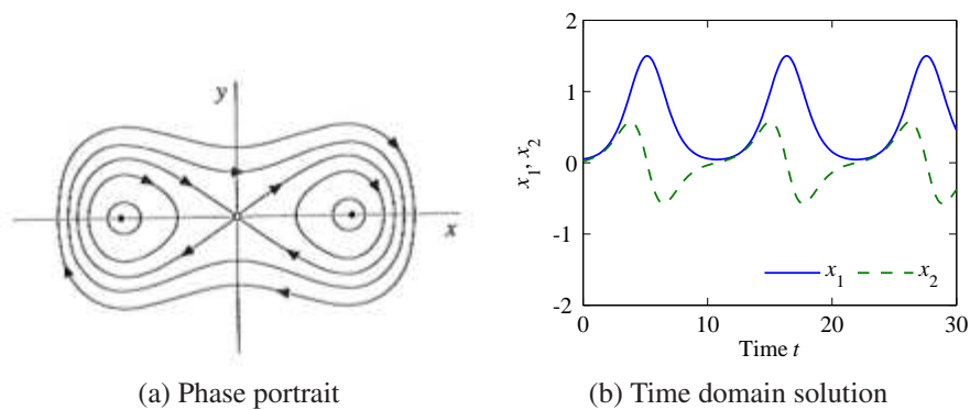
Figure 3.17: Example of a homoclinic orbit.
