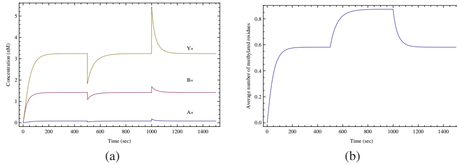
Figure 5.18: Simulation and analysis of reduced-order chemotaxis model. The parameters are taken from Rao et al. [81] and given by k_0 = 50 \text{ s}^{-1}\text{nM}^{-1} , k_1 = 100 \text{ s}^{-1}\text{nM}^{-1} , k_3 = 30 \text{ s}^{-1}\text{nM}^{-1} , k_2 = 30 \text{ s}^{-1}\text{nM}^{-1} , a = 50 \text{ s}^{-1}\text{nM}^{-1} , d = 19 \text{ s}^{-1} , and k_4 = 1 \text{ s}^{-1} . The concentrations are R_{\text{tot}} = 0.2 \text{ nM} , \sum_{i=0}^4 T_i = 5 \text{ nM} , A_{\text{tot}} = 5 \text{ nM} , B_{\text{tot}} = 2 \text{ nM} , and Y_{\text{tot}} = 17.9 \text{ nM} . Also, we have k_B = 0.5 \text{ s}^{-1} , K_B = 5.5 \text{ nM} , k_R = 0.255 \text{ s}^{-1} , and K_R = 0.251 \text{ nM} .
