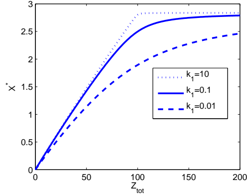
Figure 2.26: Steady state characteristic curve of the phosphotransfer system. Here, we have set k_2 = k_3 = 0.1 \text{ s}^{-1} , k_4 = 0.1 \text{ nM}^{-1} \text{ s}^{-1} , \pi_1 = \pi_2 = 3.1 \text{ s}^{-1} , and X_{\text{tot}} = 100 \text{ nM} .
