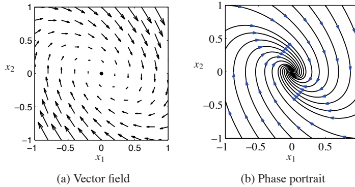
Figure 4.3: Phase portraits. (a) This plot shows the vector field for a planar dynamical system. Each arrow shows the velocity at that point in the state space. (b) This plot includes the solutions (sometimes called streamlines) from different initial conditions, with the vector field superimposed.
