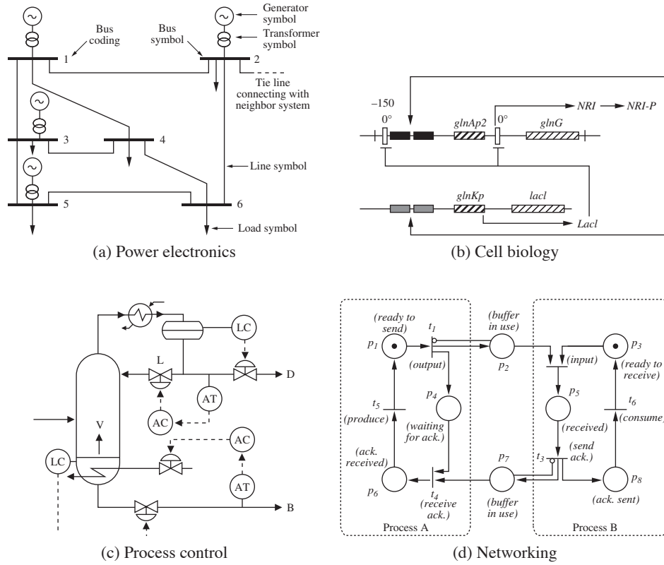
Figure 2.11: Schematic diagrams for different disciplines. Each diagram is used to illustrate the dynamics of a feedback system: (a) electrical schematics for a power system [131], (b) a biological circuit diagram for a synthetic clock circuit [22], (c) a process diagram for a distillation column [177] and (d) a Petri net description of a communication protocol.
