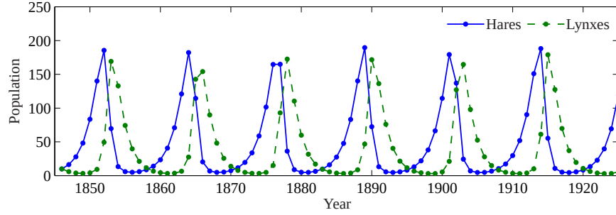
Figure 2.7: Discrete-time simulation of the predator-prey model (2.13). Using the parameters a = c = 0.014 , b_f(u) = 0.6 and d = 0.7 in equation (2.13) with daily updates, the period and magnitude of the lynx and hare population cycles approximately match the data in Figure 2.6.
