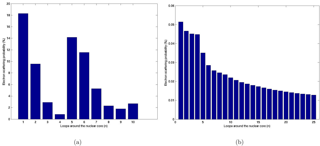
Fig. 11. The 3-degree of freedom Rydberg atom in crossed fields for \epsilon = 0.58 . Approximation of transport probabilities in (a) the full scattering problem and (b) the half scattering problem.
