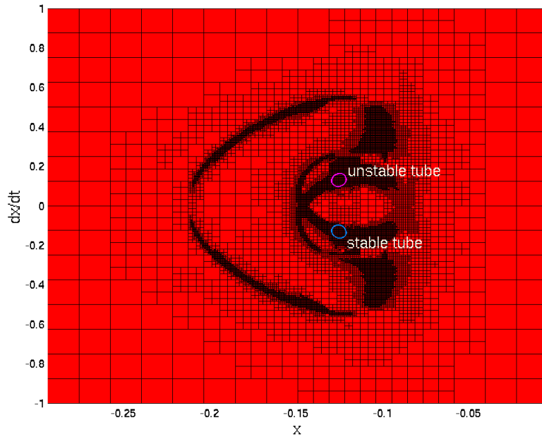
Fig. 8. Adaptive box covering for the Rydberg atom in crossed fields. In the 2-degree of freedom system for \epsilon = 0.57765 those boxes are refined that contribute to the error in the computation of the transport rates. The unstable and stable tube intersections are superimposed.
