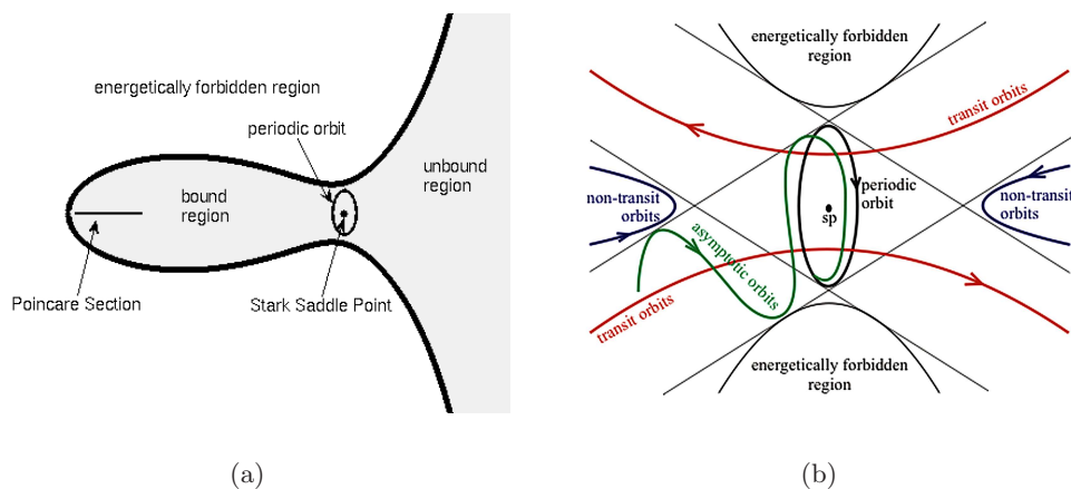
Fig. 1. (a) xy projection of the Hill's region (schematic). (b) The possible types of trajectories in the equilibrium region are shown in the xy projection (schematic). There are three different types of orbits — asymptotic, transit and non-transit orbits (see [21]).
