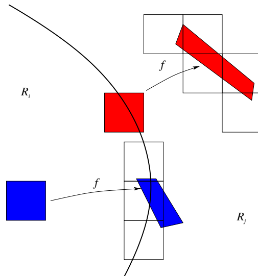
Fig. 7. Two box transitions that contribute to the error between the computed and the actual value of the transport rate from a region R_i into region R_j after one iterate. Picture taken from [12].
