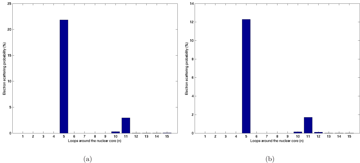
Fig. 10. Full scattering problem for the Rydberg atom in crossed fields for \epsilon = 0.57765 . Approximate transport probabilities \tilde{q}_{1,2}(n) for n = 1, \dots, 15 in (a) the 2-degree of freedom system and (b) the 3-degree of freedom system.
