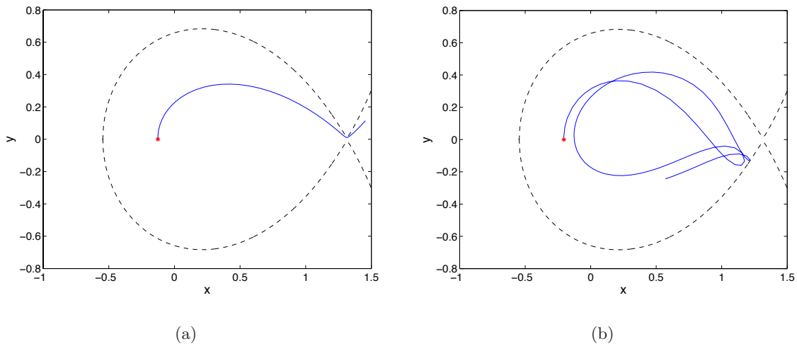
Fig. 2. Typical (a) transit and (b) nontransit trajectories. The xy projection of the Hill's region is shown as the dotted line. Compare with Figure 1.
