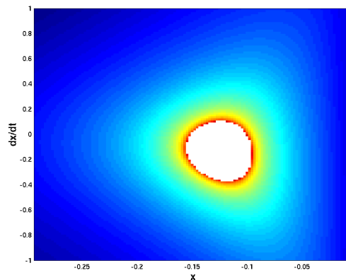
Fig. 5. First return time distribution of the rectangle X = [-0.295, -0.005] \times [-1.0, 1.0] for an electric field parameter \epsilon = 0.58 . The white region in the middle indicates an infinite return time meaning points in this region do not come back to the Poincaré section under consideration and the other shades correspond to a finite return time decreasing from the inner to the outer region.
