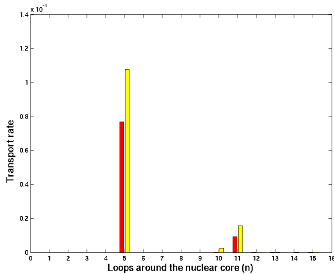
Fig. 9. Full scattering problem for the 2-degree of freedom Rydberg atom in crossed fields for \epsilon = 0.57765 . Approximations of the lower bound \underline{T}_{1,2}(n) (dark bar) and the upper bound \overline{T}_{1,2}(n) (light bar) on the transport rate for n = 1, \dots, 15 are shown.
