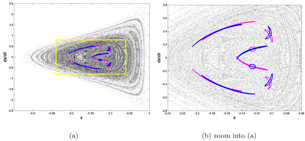
Fig. 3. Chaotic sea for the 2-degree of freedom Rydberg atom is shown with the first six intersections of the unstable (light) and stable (dark) tube boundaries with the Poincaré section \Sigma under consideration. For this electric field parameter of \epsilon = 0.57765 , the neck between the bound and unbound region is only open a little.
