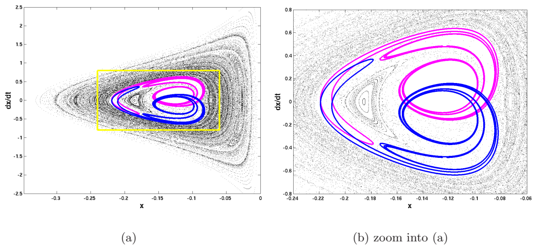
Fig. 4. Chaotic sea for the 2-degree of freedom Rydberg atom for an electric field parameter of \epsilon = 0.58 . The first three intersections of the unstable (light) and stable (dark) tube boundaries with the Poincaré section \Sigma under consideration are shown in (a), whereas (b) is a zoom into the interesting region of (a).
