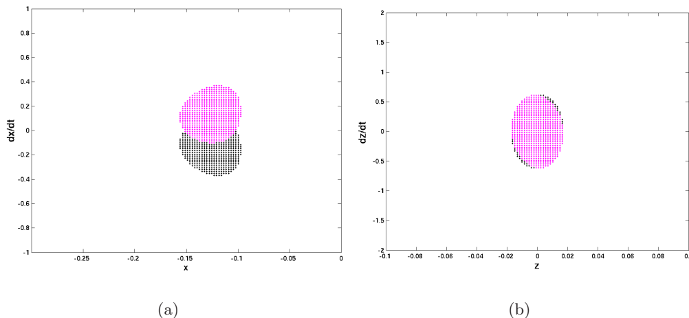
Fig. 6. First intersection of the stable (dark) and unstable (light) tube with the Poincaré section in (a) x\dot{x} - and (b) z\dot{z} -projections for a parameter value \epsilon = 0.58 .
