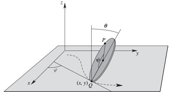
Figure 2. The geometry for the rolling disk.
