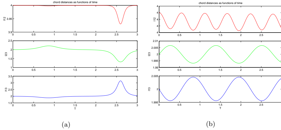
Fig. 1. – Chord distances as functions of time. Great circle relative equilibrium. (a) Unstable, \Gamma_1 = 3, \Gamma_2 = 2, \Gamma_3 = 0.2, \det \delta^2 H_\xi = -1 ; (b) Stable, \Gamma_1 = 3, \Gamma_2 = 2, \Gamma_3 = 0.02, \det \delta^2 H_\xi = 0.8 .
