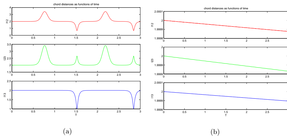
Fig. 2. – Chord distances as functions of time. Equilateral triangle relative equilibrium. (a) Unstable, \Gamma_1 = 2, \Gamma_2 = 1, \Gamma_3 = -2, \det \delta^2 H_\xi = -4 ; (b) Stable, \Gamma_1 = 2, \Gamma_2 = 1, \Gamma_3 = 4, \det \delta^2 H_\xi = 14 .
