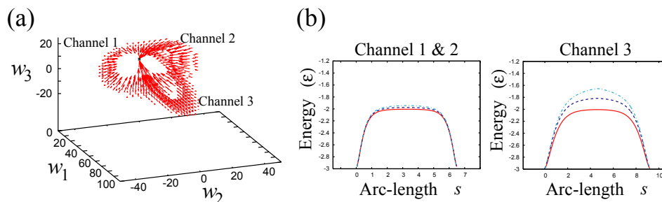
Figure 2. (a) Field of the averaged fictitious force in Hill's region at E = -1.4\epsilon . (b) Solid lines are the original potential for respective reaction channels. The broken lines and the dotted lines are the reaction-path potential at total energy E = -1.8\epsilon and E = -1.4\epsilon respectively.
