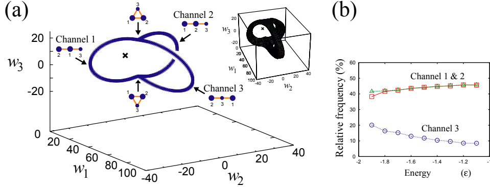
Figure 1. (a) Two equilibrium configurations and three saddle configurations of the modified M_3 cluster. The curves are the steepest descent paths of the potential energy. The two equilibrium points are located at (w_1, w_2, w_3) = (15.429, 0, \pm 13.607) . The saddle point for Channel 1 is at (10.277, 23.548, 0) while that for Channel 2 is located at (10.277, -23.548, 0) . The saddle point for Channel 3 is at (71.939, 0, 0) . Inset is the equi-potential surface at V = -1.4\epsilon . (b) Energy dependence of relative reaction frequency for each channel.
