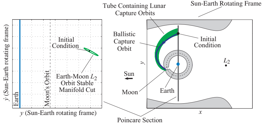
Figure 5. (a) The stable manifold cut of an Earth-Moon L_2 orbit in the Poincaré section of the Sun-Earth system. (b) A point interior to this cut, with the correct phasing of the Moon, will reach the Moon's ballistic capture region when integrated forward.
