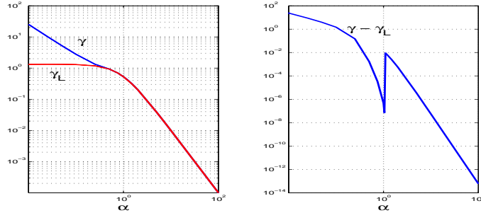
Figure 7: \gamma and \gamma_L as a function of \alpha (left) and \gamma - \gamma_L (right)
