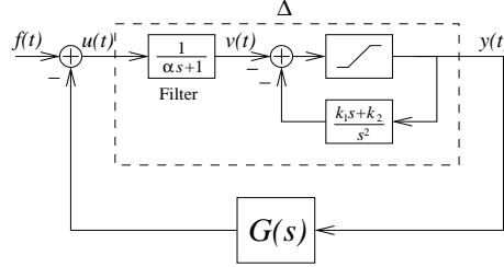
Figure 4: Loop transformation with stable operators
