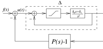
Figure 3: Loop transformation with an unstable operator \Delta
