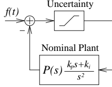
Figure 2: Nominal system and uncertainty
