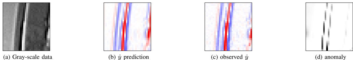
Figure 10. Example of failure for very fine details . We noticed that the detection would give false positives for very fine textures. This figure shows a blowup of a 16\text{px} \times 16\text{px} detail of a door frame. The observed derivative and the prediction are apparently a very close match, but a closer examination reveals that the prediction is shifted 1 pixel to the left. Subfigure (d) shows the detection signal: because of the 1 pixel inconsistency, two bands are detected as inconsistent. We do not have a full explanation of this phenomenon, but probably it is linked to the fact that we approximate the derivative at instant k using the the difference y_k - y_{k-1} , thus introducing a phase delay.
