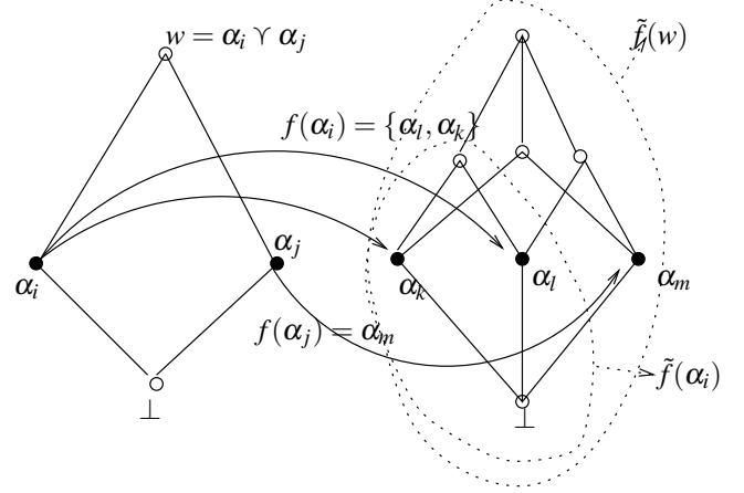
Fig. 1. Extension \tilde{f} on lattice \chi .
