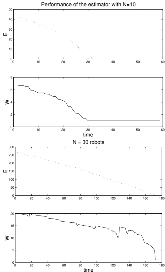
Fig. 3. Example with N=10 (up) and N=30 (down). Dashed plots show the stabilization function of the \alpha assignment (E). Solid plots show the function W for the estimator.
