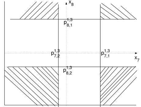
Fig. 2. Dashed regions are the ones where g_{1,3} is true.
