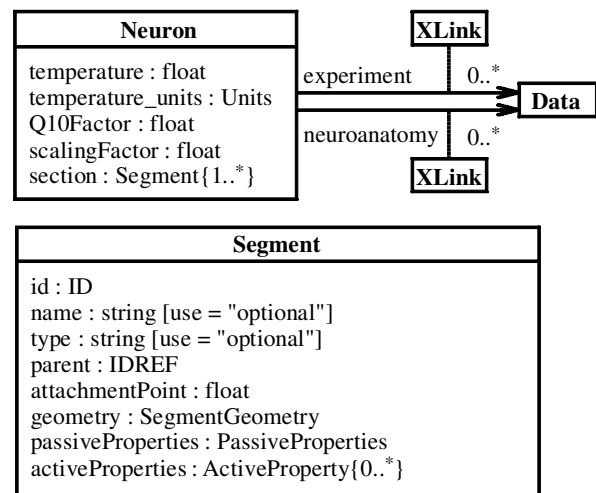
Figure 16. The Neuron template.
