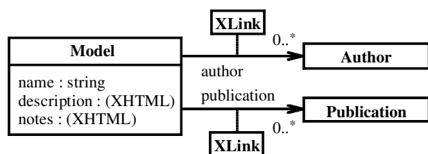
Figure 8. The Model template.
