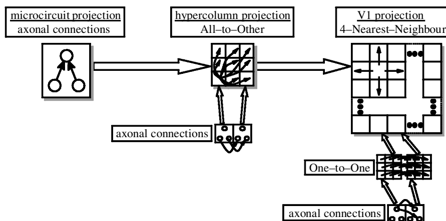
Figure 13. A set of hierarchical populations: the microcircuit is described with simple axonal connections; the hypercolumn is described as an all-to-other projection between microcircuits, where each link in the projection is the bundle of axonal connections shown below; V1 is described as a four-nearest-neighbour projection between hypercolumns, where each link in the projection is another projection, one-to-one, between microcircuits in the hypercolumns, and each link in the one-to-one projection is the bundle of axonal connections shown below.
