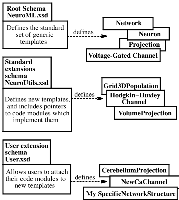
Figure 3. Overview of the organization of XML schemas in this approach.
