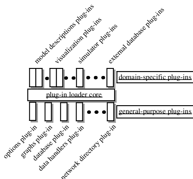
Figure 1. The component-based architecture: many components use NeuroML to communicate. The same plug-in loader is used for domain-specific plug-ins as for the library of general purpose plug-ins.
