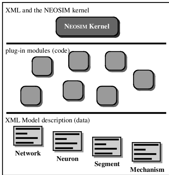
Figure 17. The NEOSIM kernel uses a number of declarative model description levels, given in different XML files. Extra code features are introduced using plug-in modules.
