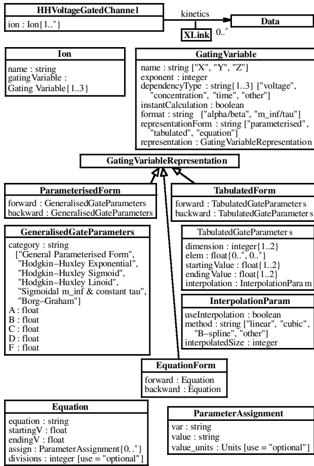
Figure A1. The definition of the HHVoltageGatedChannel template.
