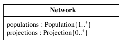
Figure 9. The Network template includes a number of Neuron populations and a number of Projections (possibly zero) between populations.
