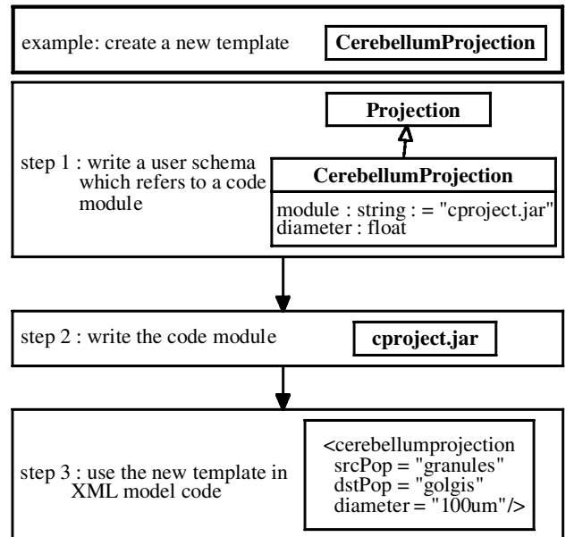
Figure 4. The steps involved in adding a new user template with an associated code module and using it. First, the template describing the interface to the code module is defined. Second, the code module is written. Third, the new template is used in a model description.
