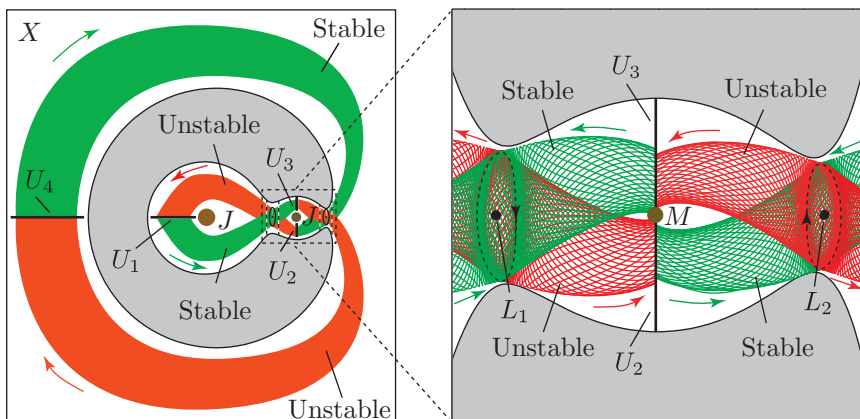
FIGURE 9.4.1. Location of libration point orbit invariant manifold tubes in position space. Stable manifolds are lightly shaded, unstable manifolds are darkly. The location of the Poincaré sections ( U_1 , U_2 , U_3 , and U_4 ) are also shown.
