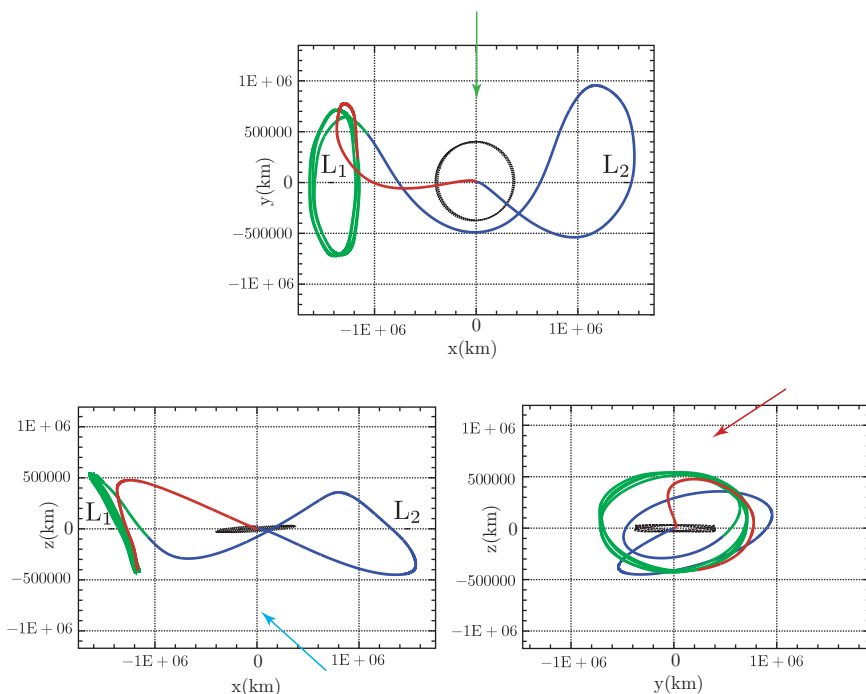
FIGURE 1.2.7. The xy , xz , and yz projections of the three-dimensional Genesis trajectory shown in the preceding figure.
