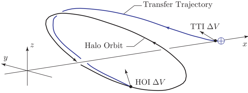
FIGURE 7.3.1. The Launch Problem: finding the best solution from Transfer Trajectory Insertion (TTI) to Halo Orbit Insertion (HOI).
